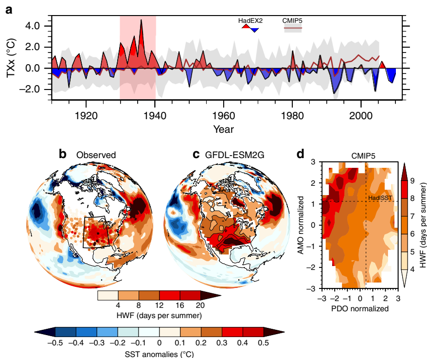
Fig. 1 Observed and simulated central US summer heatwave activity and associated sea surface temperatures. a Observed summer (June–August) maximum daily maximum temperature ( T_{xx} ) anomalies (relative to 1901–2010) averaged over the central US (box in b ), from gridded observations (HadEX2; colour), and 20 Coupled Model Intercomparison Project Phase 5 (CMIP5) historical model simulations (grey line with shading indicating the 10–90th percentile range; relative to 1901–2005). b, c Summer sea surface temperature anomaly and heatwave frequency (HWF) patterns averaged across the most active heatwave summer decade (11 years) per century over the central US for station observations ( b ; pink shade in a ), and a selected CMIP5 model (Geophysical Fluid Dynamics Laboratory Earth System Model with Generalised Ocean Layer Dynamics component, GFDL-ESM2G) decade with heatwave activity commensurate with observations ( c ). d Composite anomalies of central US summer HWF as a function of the normalised annual Pacific Decadal Oscillation (PDO) and Atlantic Multidecadal Oscillation (AMO) indices, from 22 CMIP5 pre-industrial (pi) Control experiments totalling 10,900 years (1930s decadal observations shown as the intersect of dotted lines). The PDO and AMO definition are described in the ‘Methods’.
