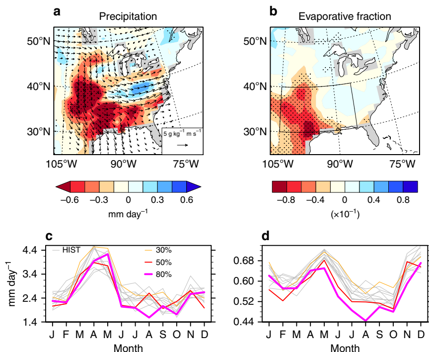
Fig. 4 Late spring conditions prior to the Dust Bowl summers. a, b , Composite differences in April–May conditions between the five-member Atlantic sea surface temperature (SST) ensemble mean (ATL HIST ) and five-member Pacific SST ensemble mean (PAC HIST ) prior to the Dust Bowl summers for 1930–37. The fields shown are precipitation (colours; a ) and 850 hPa moisture flux (vectors; a ) and evaporative fraction ( b ). Stippling on precipitation and evaporative fraction contours indicates significance above the 95% confidence level based on a bootstrap mean difference on 10,000 × 8 April–May samples (resampled). c, d Annual cycle of precipitation ( c ) and evaporative fraction ( d ) for the ten-member historical SST members (HIST) and bare-soil model experiments averaged over 1930–1937 and the southern-central US (region in (b); 105°–85°W, 30°–40°N).
