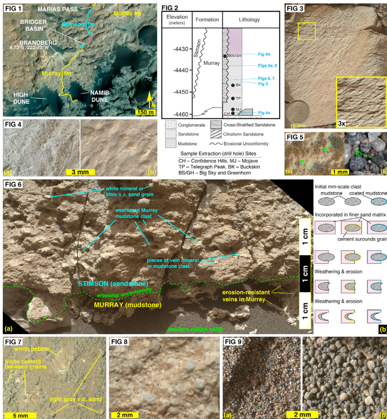
Fig 1. Curiosity's May–Dec. 2015 traverse between Marias Pass and Namib Dune . Base map is from NASA/JPL ( http://mars.jpl.nasa.gov/msl/mission/whereistherovernow/ ). Fig 2. Stratigraphic column for Murray/Stimson section investigated Sept. 2014 – Dec. 2015. Stratigraphic position of MAHLI images in Figs 3–8 are indicated. Fig 3. Fine laminae in Murray target Lamoose , MAHLI 1041MH0001900010400213C00. Fig 4. Qualitative mudstone color comparison in Dust Removal Tool (DRT) brushed spots; (a) light gray mudstone at Topanga ; MAHLI 0815MH0003690000301483R00; (b) purple-hued mudstone at Augusta , MAHLI 1157MH0002270000402460R00. Fig 5. (a) Lithic fragment sand grains with phenocrysts (p) in Stimson formation eolian sandstone Ledger , portion of MAHLI image 1092MH0003350020401017C00; (b) For comparison at same scale, phenocrysts in basalt eolian sand from Christmas Lake Valley, Oregon. Fig 6. (a) MAHLI Sol 1032 mosaic at Stimson-Murray contact at site named Clark . (b) Clasts composed of Murray mudstone were incorporated into the lower Stimson sands at this site; sketch shows 3 working hypotheses for nature of the mudstone clasts. Fig 7. Night view of white clasts and cements in Stimson sandstone at Big Arm ; MAHLI 1028MH0004450030204885C00. Fig 8. Stimson sandstone Ivanhoe within fracture-associated diagenetic halo; MAHLI 1092MH0001700000401028R00. Fig 9. Eolian sands of the Bagnold dune field near High Dune on Sol 1182; (a) The bulk sediment is very fine to fine sand overlain by (b) a ~1-grain-thick lag of medium to coarse sand. Grain color, shape, luster, etc., attest that a variety of mineral and lithic fragments are present.
