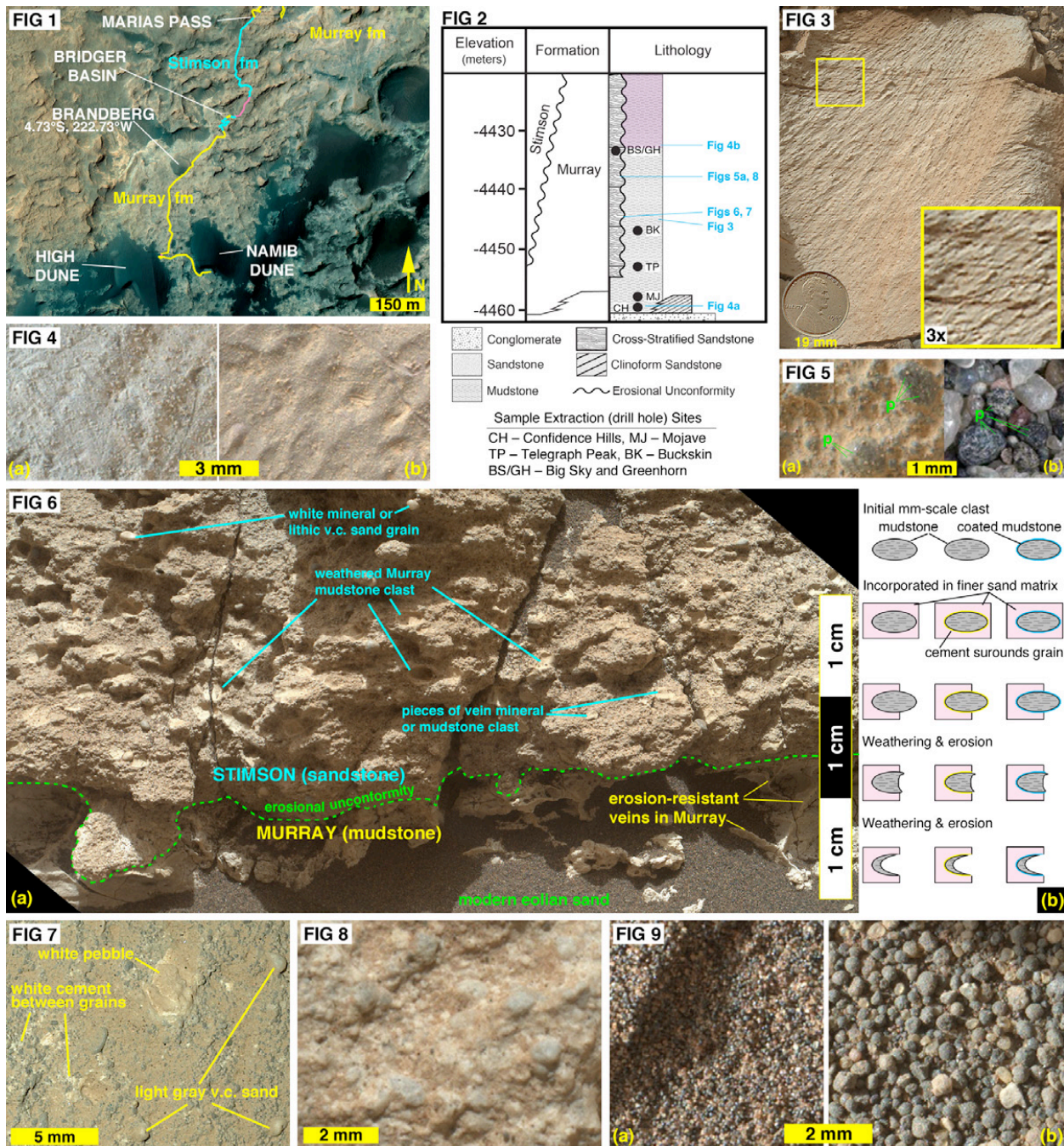
Fig 1. Curiosity's May–Dec. 2015 traverse between Marias Pass and Namib Dune . Base map is from NASA/JPL ( http://mars.jpl.nasa.gov/msl/mission/whereistherovernow/ ). Fig 2. Stratigraphic column for Murray/Stimson section investigated Sept. 2014 – Dec. 2015. Stratigraphic position of MAHLI images in Figs 3–8 are indicated. Fig 3. Fine laminae in Murray target Lamoose , MAHLI 1041MH0001900010400213C00. Fig 4. Qualitative mudstone color comparison in Dust Removal Tool (DRT) brushed spots; (a) light gray mudstone at Topanga ; MAHLI 0815MH0003690000301483R00; (b) purple-hued mudstone at Augusta , MAHLI 1157MH0002270000402460R00. Fig 5. (a) Lithic fragment sand grains with phenocrysts (p) in Stimson formation eolian sandstone Ledger , portion of MAHLI image 1092MH0003350020401017C00; (b) For comparison at same scale, phenocrysts in basalt eolian sand from Christmas Lake Valley, Oregon. Fig 6. (a) MAHLI Sol 1032 mosaic at Stimson-Murray contact at site named Clark . (b) Clasts composed of Murray mudstone were incorporated into the lower Stimson sands at this site; sketch shows 3 working hypotheses for nature of the mudstone clasts. Fig 7. Night view of white clasts and cements in Stimson sandstone at Big Arm ; MAHLI 1028MH0004450030204885C00. Fig 8. Stimson sandstone Ivanhoe within fracture-associated diagenetic halo; MAHLI 1092MH0001700000401028R00. Fig 9. Eolian sands of the Bagnold dune field near High Dune on Sol 1182; (a) The bulk sediment is very fine to fine sand overlain by (b) a ~1-grain-thick lag of medium to coarse sand. Grain color, shape, luster, etc., attest that a variety of mineral and lithic fragments are present.
