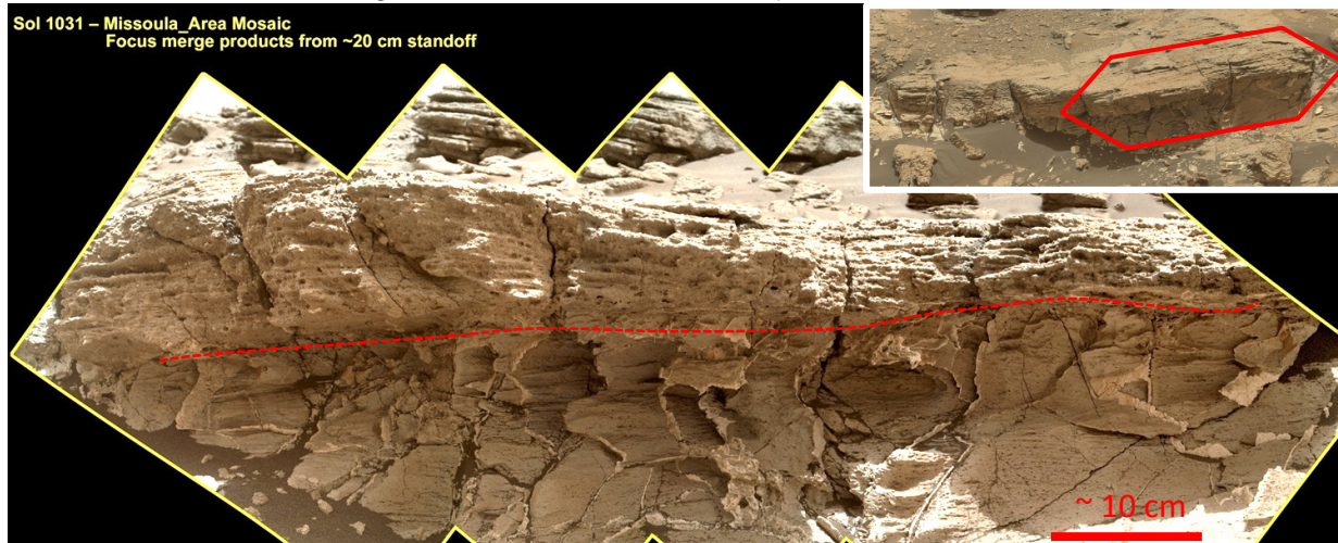
Fig. 1 MAHLI image mosaic of a portion of the Missoula/Ronan outcrop with Murray/Stimson contact (red dashed line). The image perspective from the arm camera is a “dog’s eye” view. Inset Mastcam image of the outcrop, with MAHLI location.
