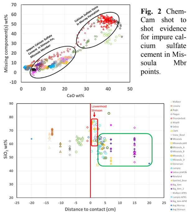
Fig. 3 ChemCam LIBS and APXS \text{SiO}_2 analyses of materials above and below the contact.
