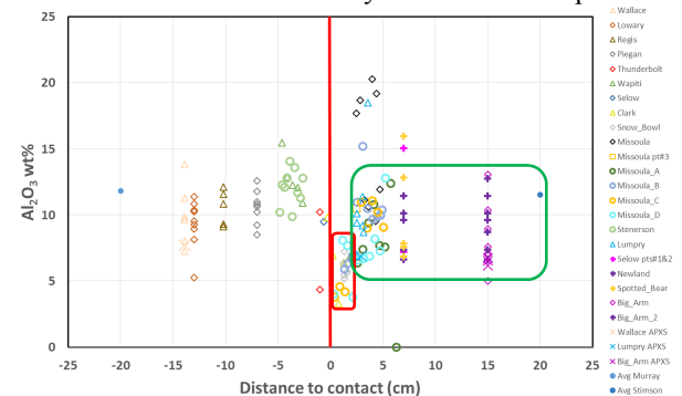
Fig. 4 ChemCam LIBS and APXS \text{Al}_2\text{O}_3 analyses of materials above and below the contact.
