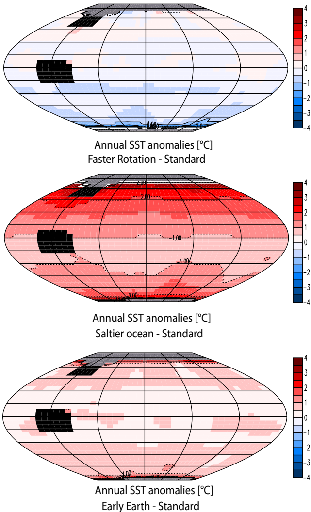
Fig. 5. Sea surface temperature anomalies ( \Delta\text{SST} ) as a result of a faster Earth rotation rate ( \text{LOD} = 16 \text{ h} ) and/or saltier ocean. Simulations performed with 3.5 Ga boundary conditions with large-droplet clouds and a \Delta F_{\text{trop}} = +24 \text{ W m}^{-2} (standard conditions). The saltier ocean experiment uses standard conditions associated with an ocean two times saltier; the faster rotation experiment has a length of day of 16 h; the early Earth experiment combines both.
