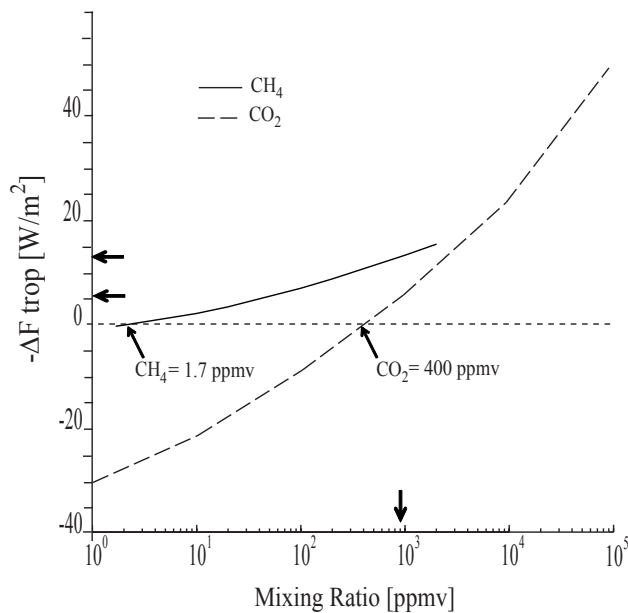
Fig. 1. Net long-wave fluxes computed for CO 2 and CH 4 with the FOAM radiative code (NCAR ccm3) (the total atmospheric is held constant, 1 bar). Thick arrows indicate the radiative forcing corresponding to 0.9 mbar of CO 2 and CH 4 . Using the present-day atmosphere as a reference, the change in net flux at the tropopause ( \Delta F_{\text{trop}} ) is 19 W m -2 , which reduces to 6 and 13 W m -2 for 0.9 mbar of CO 2 and CH 4 , respectively.
