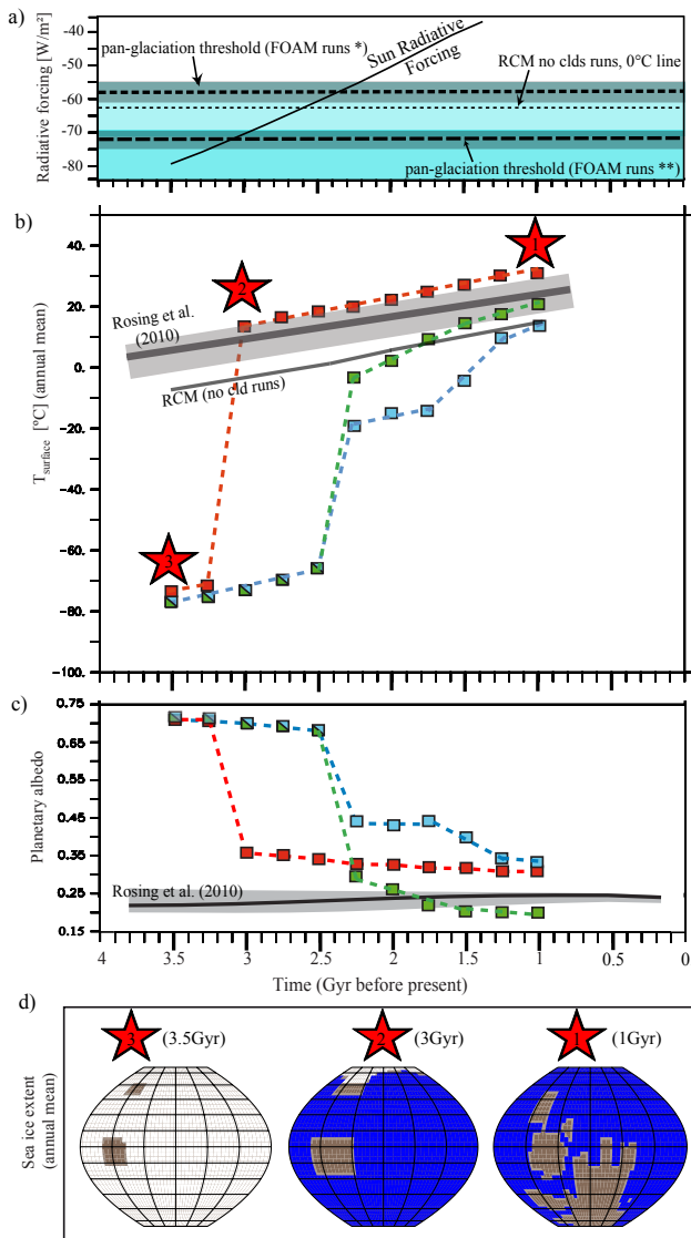
Fig. 3. 3-D climate simulations from 3.5 to 1 Ga with a greenhouse radiative forcing by \text{CO}_2 and \text{CH}_4 fixed to 19 \text{ W m}^{-2} ( \Delta F_{\text{trop}} ; see Fig. 1). (a) Radiative deficit required for the onset of a pan-glaciation with RCM (no cloud runs, surface albedo fixed to 0.264), FOAM runs (*) modern clouds and cloud-free runs and ** large-droplet clouds (20 \mu\text{m} ). Grey lines represent uncertainties related to temporal resolution (0.25 Ga). (b) Evolution of surface temperature versus time assuming increasing irradiance and linear continental growth (see Fig. 2). Grey line is from Rosing et al. (2010). Blue and red curves were obtained using liquid droplet sizes of 5 to 10 \mu\text{m} (modern clouds) and 20 \mu\text{m} (clouds with large droplets), respectively. Green squares represent the cloud-free scenario. (c) Evolution of planetary albedo versus time ( \alpha_{\text{ocean}} 0.06, \alpha_{\text{rocky desert continents}} 0.32, \alpha_{\text{seaice}} 0.5, \alpha_{\text{snow}} 0.8). (d) Red stars represent sea ice extent (white) predicted with runs performed with large (20 \mu\text{m} ) droplets (Fig. 3b, c shows the corresponding temperature/albedo).
