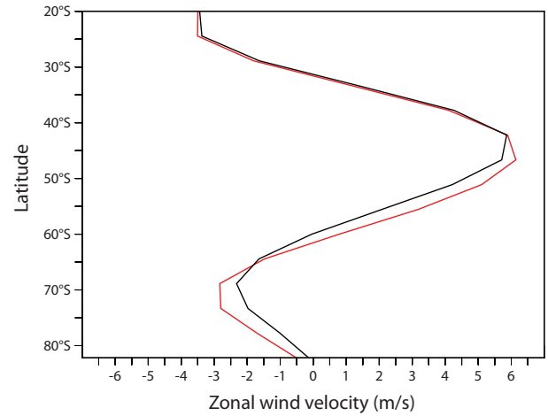
Figure 4. Zonally averaged wind velocity between 80° S and 20° S for the 560 ppm ice-free simulation (black curve) and with a large ice sheet (red curve).
