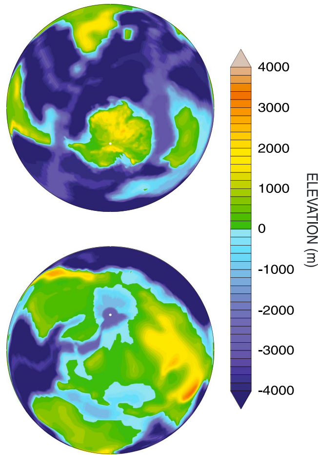
Figure 1. Early Oligocene paleogeography.
