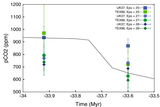
Figure 5. CO 2 data and forcing used in our EOT simulation. Data are from Pagani et al. [2011]. Blue-like colors refer to CO 2 derived from alkenones constrained with U_{37}^K , and green-like colors with TEX 86 . Estimated pCO 2 concentrations are shown with error bars for different plausible carbon isotope fractionation values (squares: \epsilon_f = 25\% , circles: \epsilon_f = 27\% , and diamonds: \epsilon_f = 28\% ).
