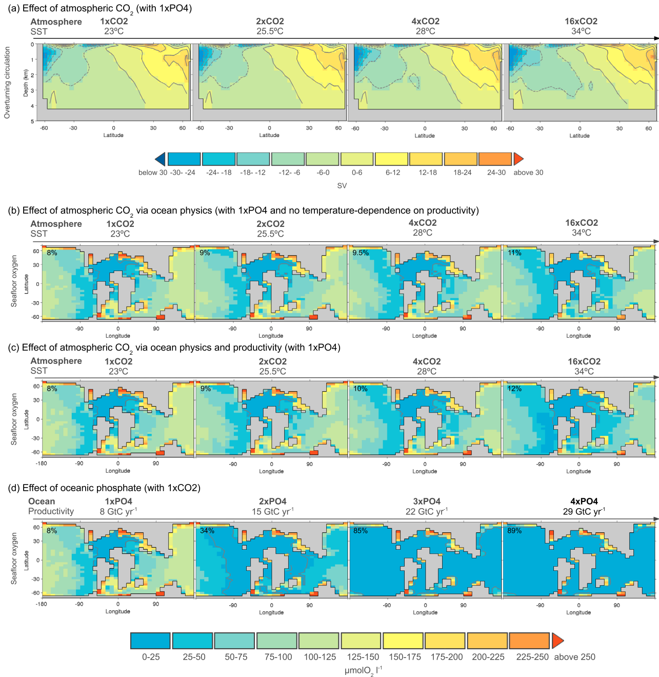
Figure 3. Model sensitivity of ocean circulation and seafloor oxygen with changing atmospheric CO 2 and oceanic phosphate (SENSITIVITY and NOBioTEMP experiments). Annual mean sea-surface temperatures (SST) are indicated for the CO 2 sensitivity experiments, and export production for the PO 4 3- sensitivity experiment. (a) Global meridional overturning circulation; (b–d) Model oxygen concentration at the seafloor. Gray contour indicates the model oxygen concentration of 10 μmol O 2 l -1 , delimiting the region of seafloor dysoxia/anoxia. The percentage of the area of seafloor dysoxia/anoxia is indicated on top of each plot. Warming temperature via higher pCO 2 does not bring about a significant change in ocean anoxia due to its small effect on oxygen solubility and ocean circulation, whereas enhanced marine productivity via higher phosphate can very quickly drive the seafloor to be anoxic.
