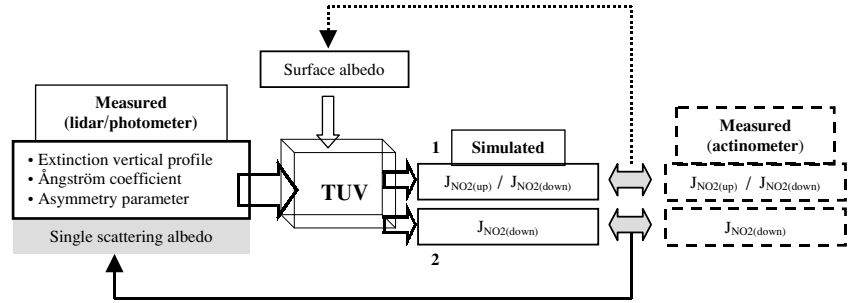
Fig 3. Schematic representation of the method used to retrieve the aerosol single-scattering albedo close to 400 nm (2) and the surface albedo (1) by iterative TUV calculations to best fit the measured values of J_{\text{NO}_2(\text{down})} and J_{\text{NO}_2(\text{up})}/J_{\text{NO}_2(\text{down})} (with an actinometer) to their values estimated by a radiative transfer model (TUV).
