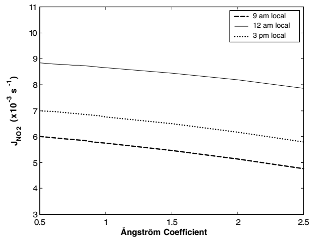
Fig. 10. Sensitivity of J_{\text{NO}_2} to variations in the Ångström coefficient at different Goa local time. The other parameters are fixed to their mean values observed during the IFP: \xi = 0.1 , \omega_0 = 0.9 , g = 0.67 and \tau_{440} = 0.72 .
