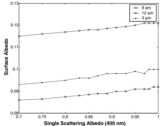
Fig 5. Surface albedo for different values of \omega_0 as retrieved at different Goa local time by iterative TUV calculations to best fit the measured and the simulated values of J_{\text{NO}_2(\text{up})}/J_{\text{NO}_2(\text{down})} . The other parameters are fixed at their mean values observed during the IFP: g = 0.67 (440 nm), \tau_{440} = 0.72 , and \text{Å} = 1.38 .
