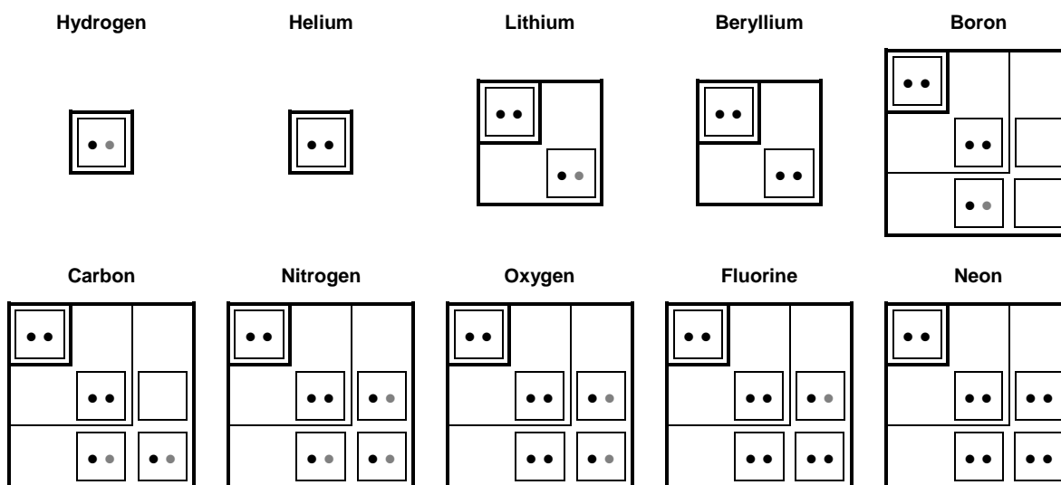
Fig. 29 Graphical quantum representation of the first ten chemical elements in chevron form design (in their ground state). See also Fig. 5 and Fig. 6.
