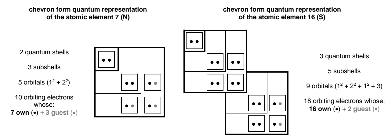
Fig. 33 Graphical quantum representation of Nitrogen and Sulphur in chevron form design (in their saturated state). See also Fig. 5 and 13.
