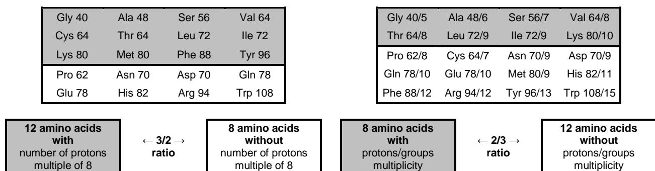
Fig. 36 Differentiation of the 20 amino acids according to the multiplicity by 8 of their number of protons (ratio: 3/2) and according to their multiplicity protons/groups (ratio: 2/3).
