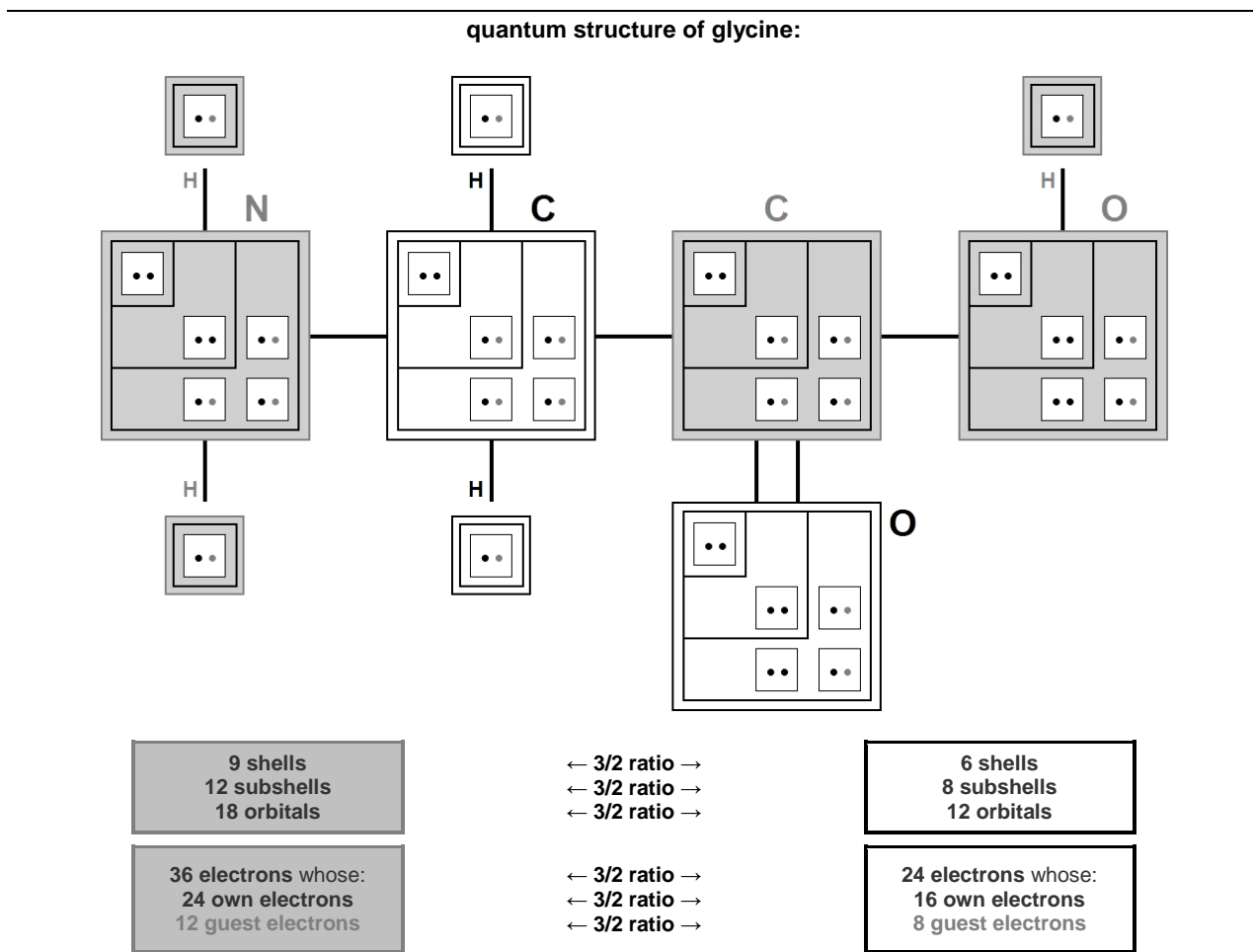
Fig. 13 Quantum structure of Glycine: 30 orbitals, 20 subshells, 15 electron shells, 60 electrons whose 40 own electrons (●) and 20 guest electrons (◐). See Fig. 5 and 9 .
