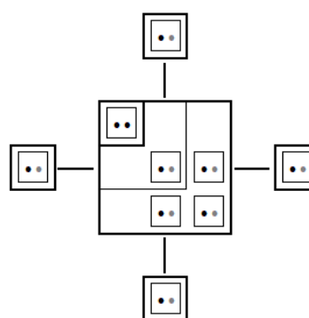
Fig. 28 Quantum configuration of carbon in excited then saturated state. See also Fig. 2 and 13 .
