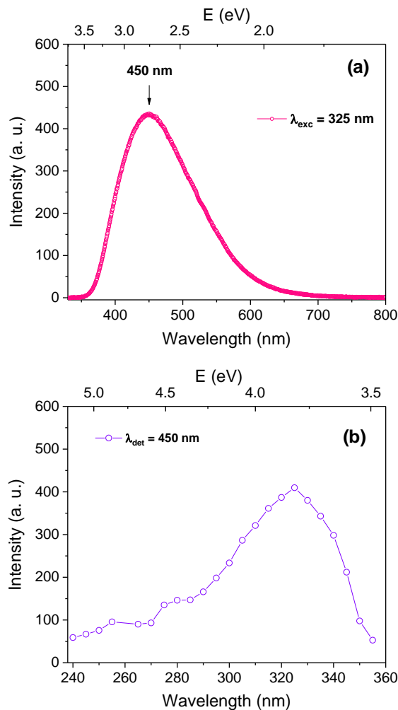
Fig. 4. (a) PL spectrum of cerium-doped air-clad optical fiber under 325 nm laser excitation. (b) Excitation spectrum at a detection wavelength of 450 nm of the same fiber.
