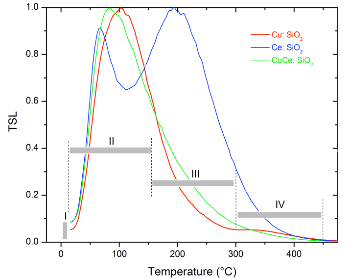
Fig. 1. TSL signal of the 3 doped sol-gel silica rods following X-ray irradiation (330 Gy ( \text{SiO}_2 )) at RT.
