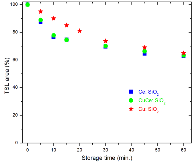
Fig. 5. Fading rate of TSL as a function of storage time in the dark of the Ce- (■), the Cu- (★) and the Ce/Cu- (●) doped rods.
