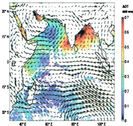
Plate 5. Mean Meteosat-5 derived AOT for (a) the last 10 days of February 1998, (b) the first, (c) the second and (d) the third period of 10 days of March 1999.
