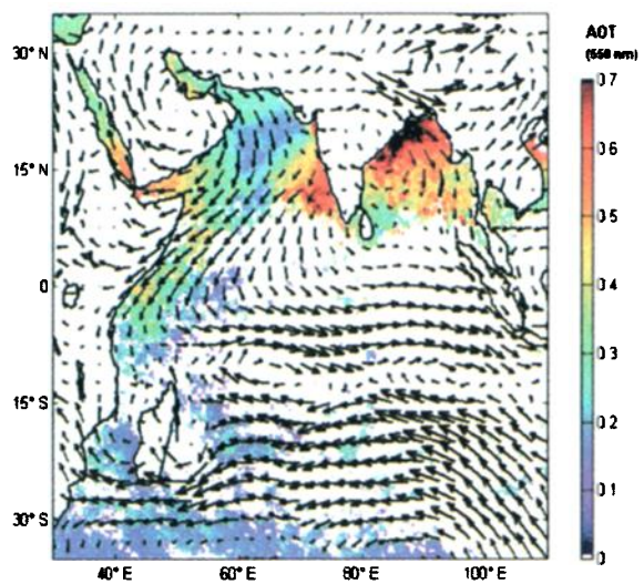
Plate 5. Mean Meteosat-5 derived AOT for (a) the last 10 days of February 1998, (b) the first, (c) the second and (d) the third period of 10 days of March 1999.
