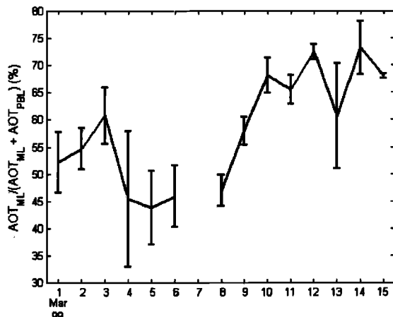
Figure 2. Ratio of the lidar-derived AOT integrated between 1 and 3 km height to the total AOT as a function of the day of the month. The vertical bars represent the associated daily range of variation.
