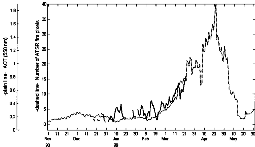
Figure 5. Moving average over 15 days of the number of fire detected by ATSR in India (area 8^{\circ} - 35^{\circ} N, 70^{\circ} - 90^{\circ} E). Data are available at http://shark1.esrin.esa.it/ionia/FIRE/ .
