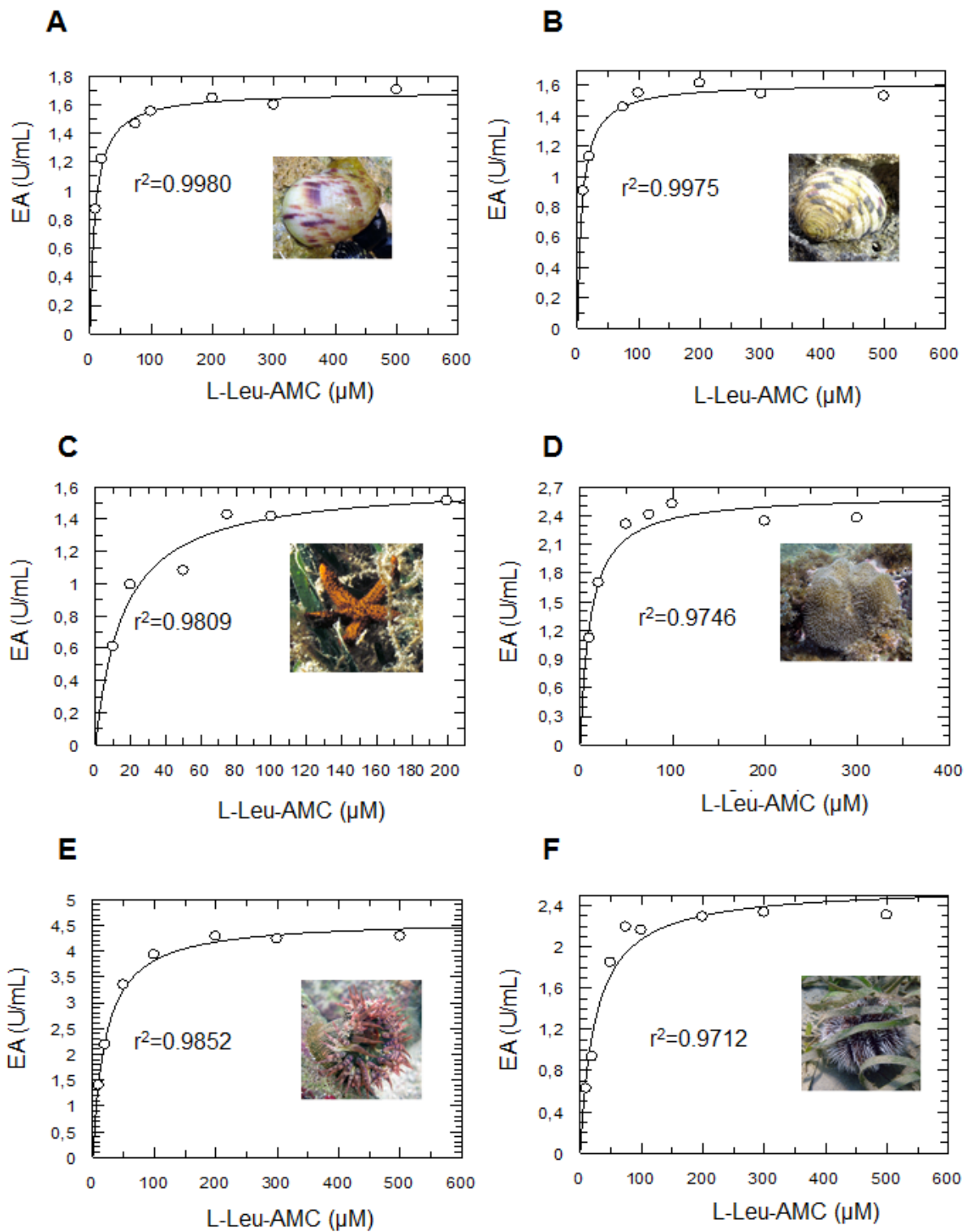
Figure 2 SM. Michaelis-Menten behavior versus L-Leu-AMC (10-500 \mu\text{M} ) of the neutral aminopeptidase-like activities detected in crude aqueous extracts from marine invertebrates. These assays were done in Tris HCl 50 mM pH 7.5, with a fixed amount of each crude extract inside the lineal range of initial rate, in a final assay volume of 200 \mu\text{L} . A: Nerita peloronta (0.42 mg/mL), B: Nerita versicolor (0.29 mg/mL), C: Echinaster (Othilia) echinophorus (0.07 mg/mL), D: Stichodactyla helianthus (0.42 mg/mL), E: Bunodosoma granuliferum (0.09 mg/mL), F: Tripneustes ventricosus (0.74 mg/mL). Pictures were kindly supplied by Professor Jose Espinosa, PhD, from the National Institute of Oceanology, CITMA, Cuba.
