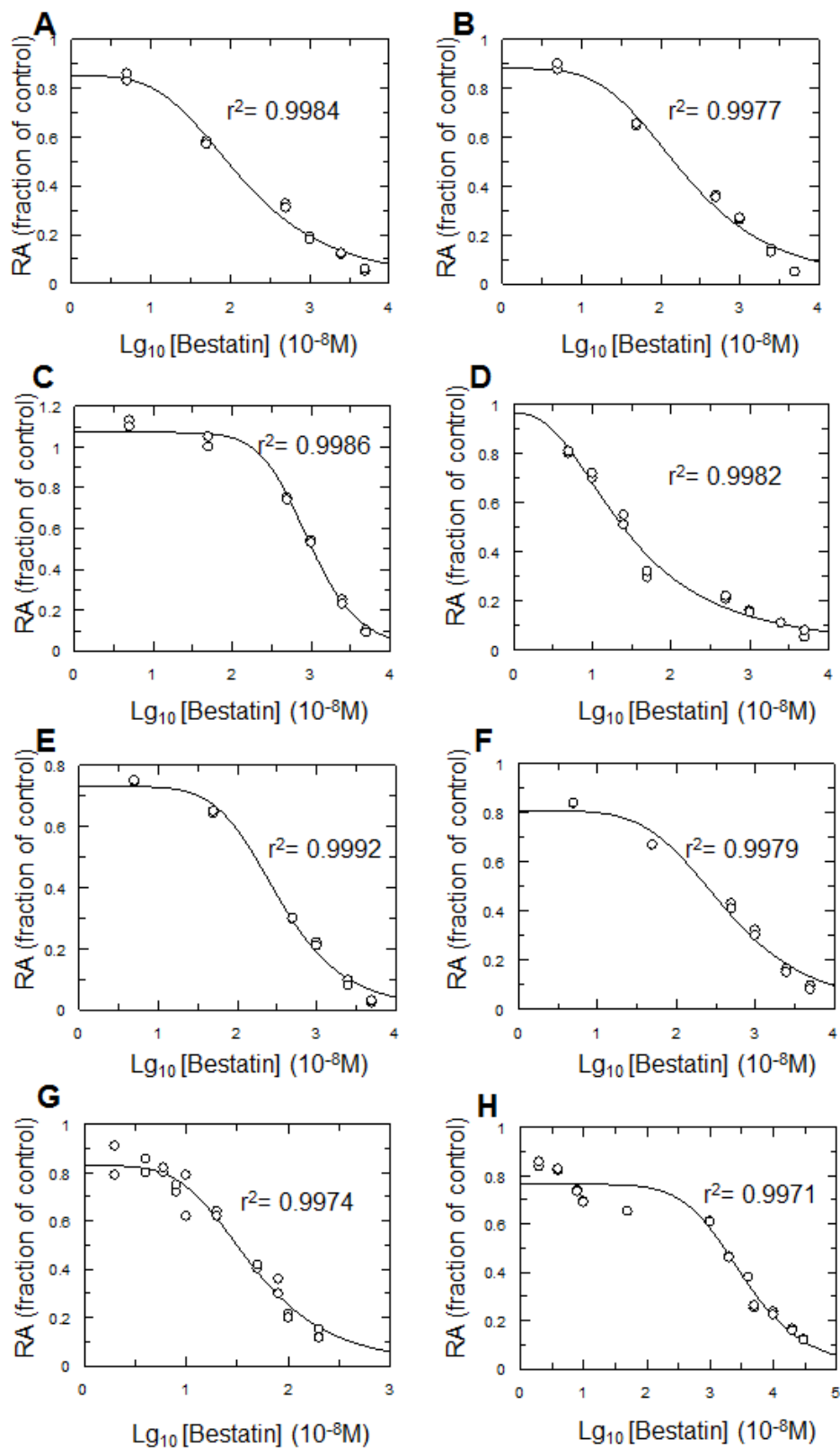
Figure 1 SM. Dose-response curves for the inhibition by bestatin (0.05-50 \mu\text{M} ) of the neutral aminopeptidase-like enzymes detected in crude aqueous extracts from marine invertebrates. These assays were done in Tris HCl 50 mM pH 7.5, with a fixed amount of each crude extract inside the linear range of initial rate, in a final assay volume of 200 \mu\text{L} . Each aqueous crude extract was preincubated for 30 min with bestatin prior to the addition of L-Leu-AMC at 0.025 mmol/L. A: Nerita peloronta (0.42 mg/mL), B: Nerita versicolor (0.29 mg/mL), C: Tripneuste ventricosus (0.74 mg/mL), D: Echinaster echinophorus (0.07 mg/mL), E: Stichodactyla helianthus (0.42 mg/mL), F: Bunodosoma granulifera (0.09 mg/mL), G: rPfA-M17 (280 nM), H: hAPN (0.25 mg/mL).
