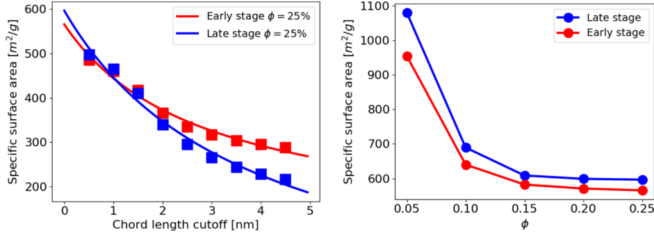
Figure 11. Left: The specific surface area as a function of the chosen chord length cutoff. By fitting the calculated data points to f(l_c) = \frac{A}{1+Bl_c} + C , we extrapolate to the l_c = 0 limit and obtain the geometric surface area S_{sp} = A + C . Right: The value for the specific surface area obtained by extrapolation for different volume fraction \phi .
