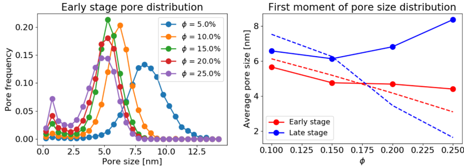
Figure 8. Left: PSD with ES potential for several volume fractions. The pore frequency describes what fraction of pore space is occupied by pores of a given radius. Right: First moment of the PSD for both potentials as a function of \phi . The solid line represents the low \mu middle region, while the dashed line is for the high \mu edge.
