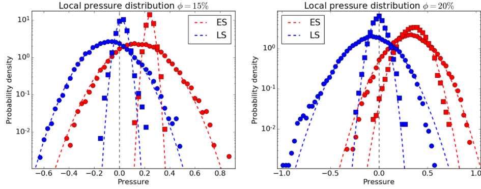
Figure 5. Distributions of local pressure at the edge (circle symbols) and center (square symbols). Gaussian fits are also plotted as dashed lines.
