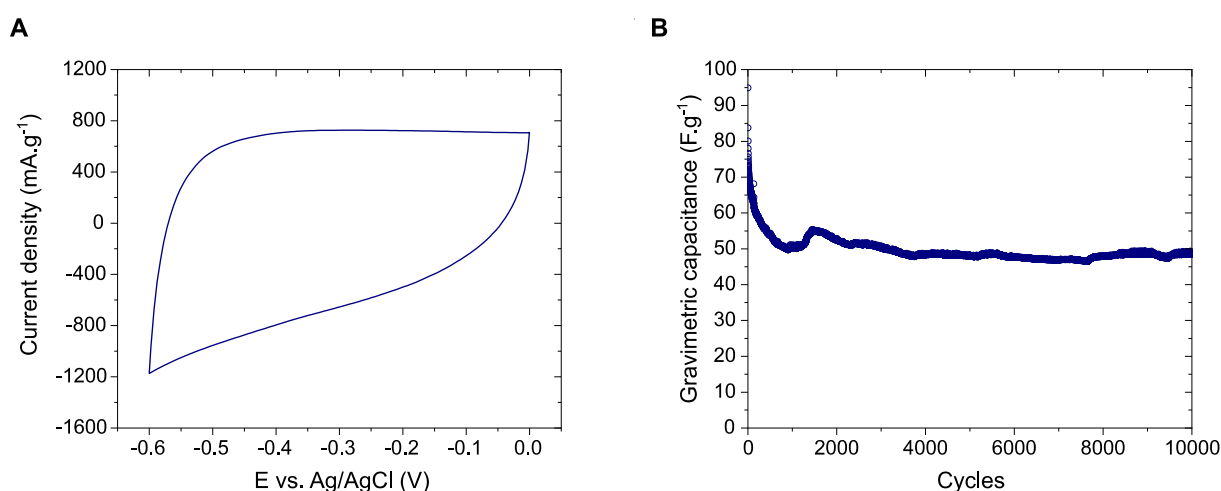
Figure S1: A) Typical voltammogram and B) Long term cycling behavior of the \text{FeWO}_4 material over 10 000 cycles. Electrolyte: 5M \text{LiNO}_3 ; Scan rate: 20 \text{ mV.s}^{-1} . The decay observed on the first 1000 cycles maybe due to a rearrangement at the surface of the particles during cycling.
