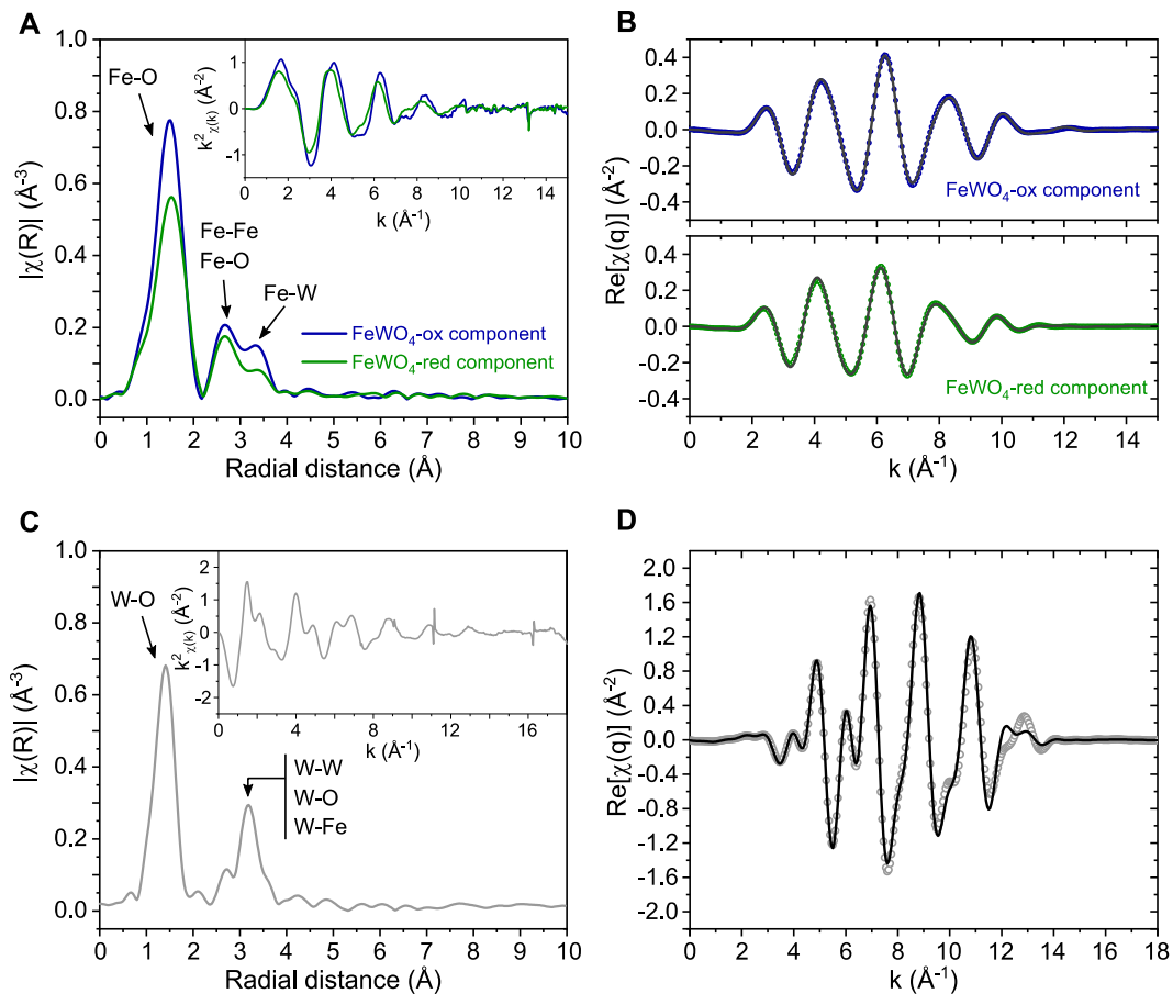
Figure 6: Magnitude of Fourier transforms of k^2 -weighted EXAFS oscillations for FeWO 4 's first cycle along with fitting results. (a, b) Principal components analysis (PCA) at Fe K-edge showing the two reconstructed principal components, i.e. FeWO 4 -ox (dark blue, pristine sample) and FeWO 4 -red (dark green, reduced electrode at -0.6 V vs. Ag/AgCl); c) W L 3 -edge spectrum, along with the fitting result (d). No structural evolution is detected at W L 3 -edge during cycling.
