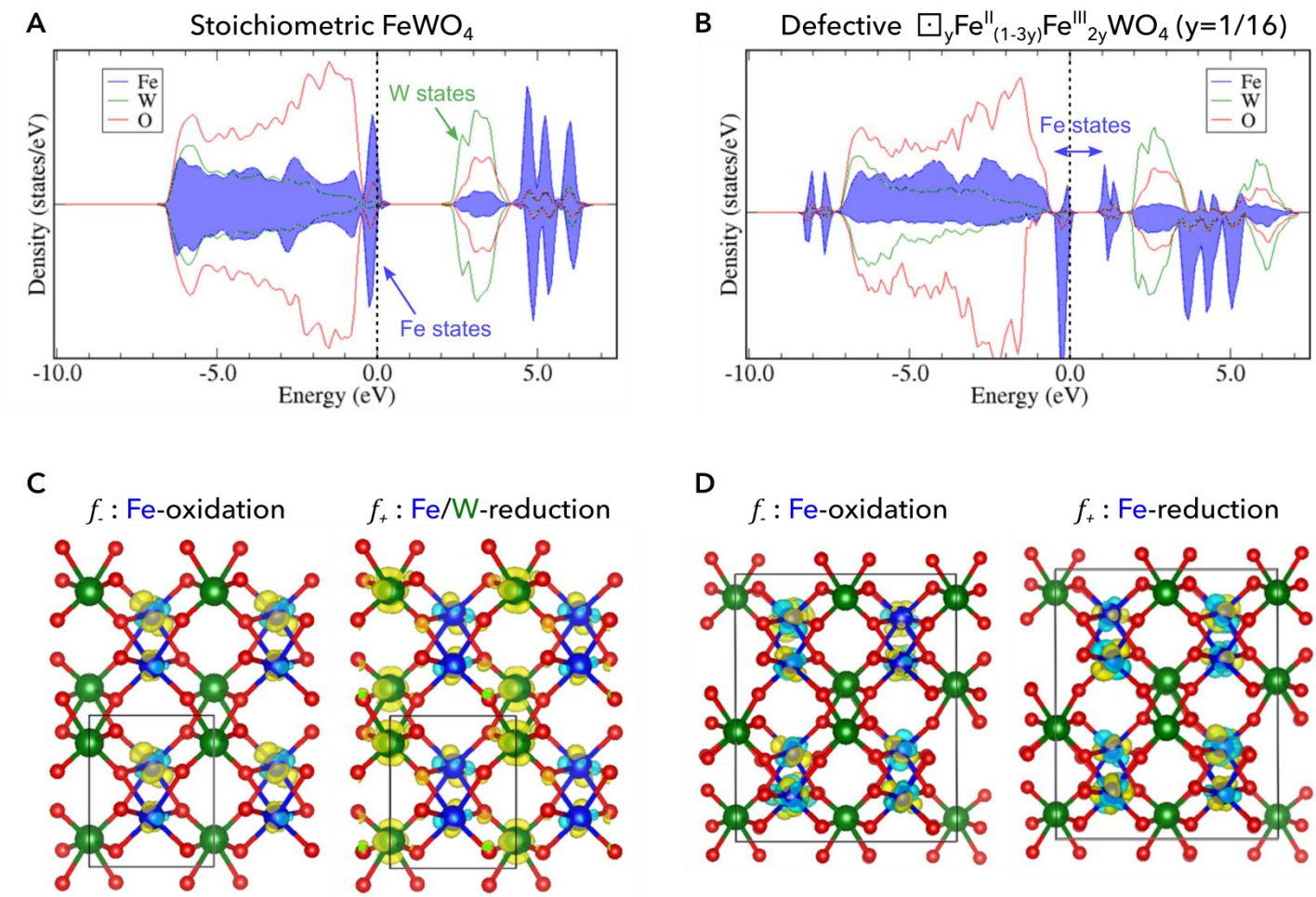
Figure S6: Atom-projected Density of states for A) stoichiometric FeWO 4 and B) Fe-defective □ y Fe II (1-3y) Fe III 2y WO 4 bulk, as well as Fukui functions f_+ and f_- for C) stoichiometric FeWO 4 and D) Fe-defective □ y Fe II (1-3y) Fe III 2y WO 4 bulk, as computed from first-principles DFT calculations in the AFM spin configuration. Iron, tungsten and oxygen are represented in blue, green and red, respectively both in the pDOS plots and in the crystal structures. The Fermi level is indicated by the vertical dotted line in the pDOS. The yellow and blue volumes of the Fukui functions represent the accumulation and depletion of charge around each atom. For the stoichiometric FeWO 4 , the pDOS shows a narrow Fe-band below the Fermi level and a wider W-band above the Fermi level. Accordingly, the Fukui functions f_- (hole addition) and f_+ (electron addition) show that Fe and W are the main centers of the oxidation (anodic scan) and reduction (cathodic scan), respectively. When Fe-vacancies are introduced in the FeWO 4 supercell (16 formula units), the splitting of the Fe-states around the Fermi level leads to a different electrochemical response of the system with Fe being the redox center of both the anodic and cathodic scans, even at very low y-content (here 1/16).
