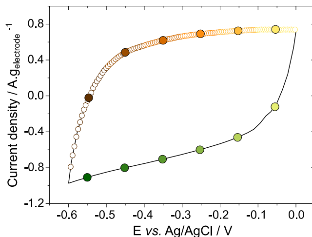
Figure 2: Cyclic voltammogram of the iron tungstate electrode cycled at 10 \text{ mV.s}^{-1} in 5\text{M LiNO}_3 aqueous electrolyte (reference electrode Ag/AgCl; counter electrode: platinum wire). The open dots represent the XAS spectra acquisition rate (1 spectrum every 0.5 s), the full dots corresponding to the average of 20 spectra for clarity purpose (1 averaged spectrum every 10 s).
