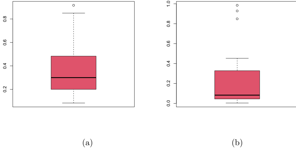
Figure 3: Boxplots of the (a) times of infection data set and (b) failure times data set.
