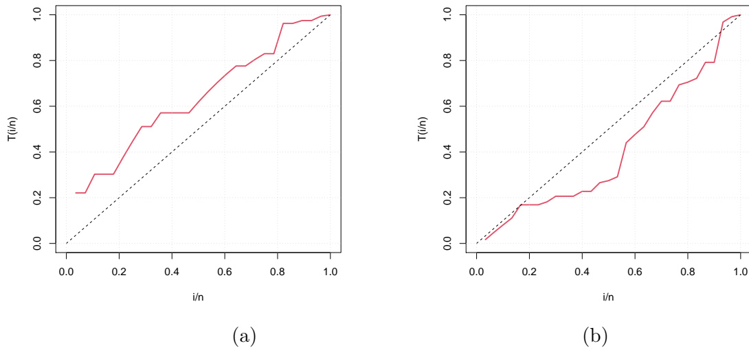
Figure 4: TTT plots of the (a) times of infection data set and (b) failure times data set.
