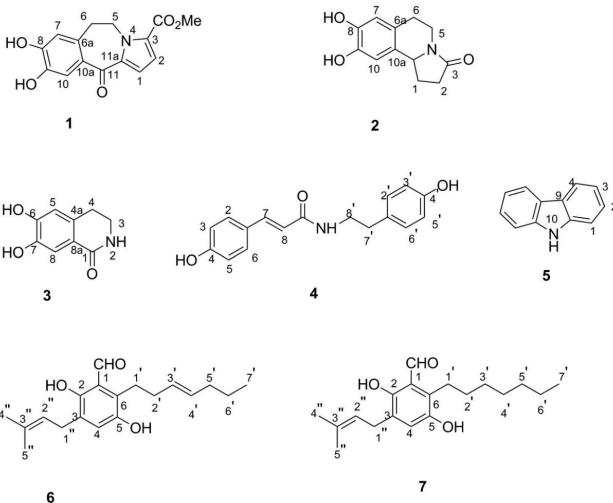
Figure 1. Structure of compounds 1–7.
