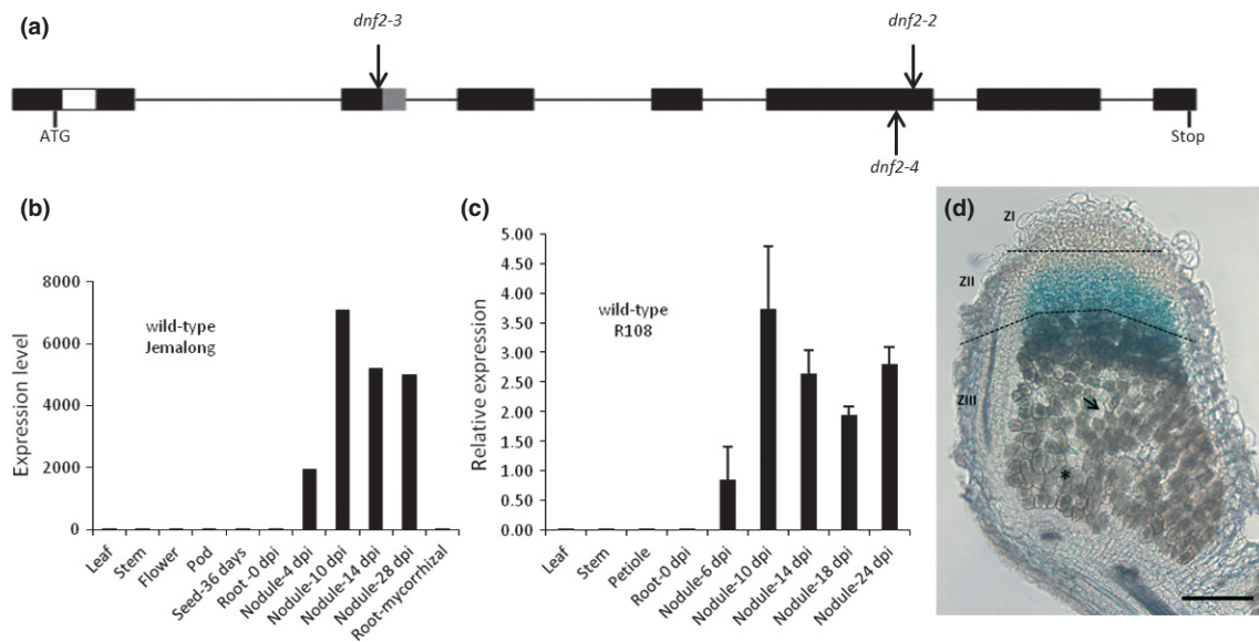
Fig. 1 DNF2 gene structure and nodule-specific gene expression. (a) The DNF2 ( MTR_4g085800 ) gene contains eight exons represented by black boxes. The gray area in the 3' part of the third exon contains four alternative splicing sites (see Supporting Information Fig. S5). The first intron that can be retained in one splicing form is represented by a white box and all other introns are represented by black lines. The positions of Tnt1 and MERE1 insertions corresponding to the three dnf2 mutant lines NF0217 ( dnf2-2 ), NF2496 ( dnf2-3 ) and MS240 ( dnf2-4 ) are indicated by black arrows (top, Tnt1 insertion; bottom, MERE1 insertion). (b) DNF2 expression profile in organs of wild-type plants from the Jemalong ecotype. Data were extracted from the MtGEA database ( http://mtgea.noble.org ). dpi, days post-inoculation. (c) Expression levels of DNF2 in different organs and during nodule formation on wild-type R108 Medicago truncatula plants. Plants were inoculated with the Sinorhizobium meliloti strain Rm41. Transcript levels were determined by quantitative reverse transcription-polymerase chain reaction (qRT-PCR) and normalized using RBP1 . Two biological replicates, one with two technical replicates, were analyzed. The error bars represent the standard error. (d) Section of a 17-dpi nodule developed on an R108 transgenic line expressing the \beta -glucuronidase gene under the control of the 4-kb DNA fragment located immediately upstream of the DNF2 predicted start codon. ZI, ZII and ZIII correspond to zones I, II and III, respectively. The asterisk and the arrow show infected and noninfected cells, respectively. Bar, 200 µm.
