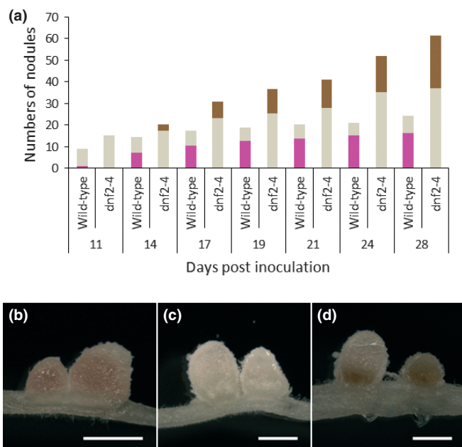
Fig. 2 Brownish nodules are produced in dnf2 . (a) The total number of nodules developed on dnf2-4 roots is higher than that on wild-type roots. Medicago truncatula wild-type and dnf2-4 nodules were counted on five pools of nine plants each. White bars, nonfixing nodules; pink bars, \text{N}_2 -fixing nodules; brown bars, brownish nodules. Note that brownish nodules are present only on the mutant line. (b) Wild-type nodules harvested 18 d post-inoculation (dpi) are pink. (c) 18-dpi dnf2-4 white nodules. (d) 18-dpi dnf2-4 nodules that have developed a brownish coloration. Bars: (b) 1 mm; (c, d) 0.5 mm. Similar results were obtained with the other two R108 mutant lines (data not shown).
