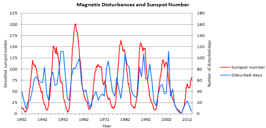
Figure 3 : Correlation between sunspot number and magnetic disturbances
