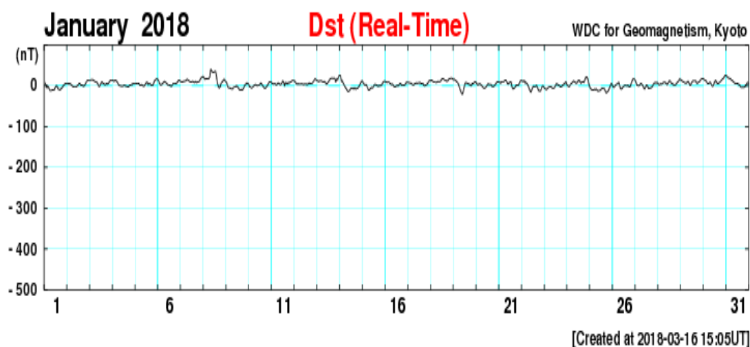
Figure 1 : Disturbance storm time index and the variations recorded in the earth's magnetic field in nano-Tesla (nT) for the month of January 2018. ( Courtesy : World Data Centre for Geomagnetism, Kyoto, Japan)
