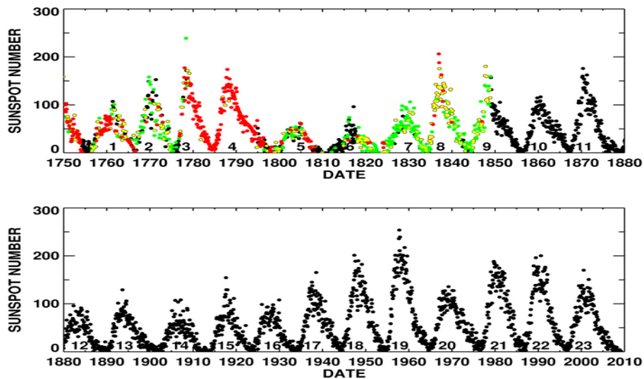
Figure 2 : Sunspot numbers shown from the year 1750 - 2010
