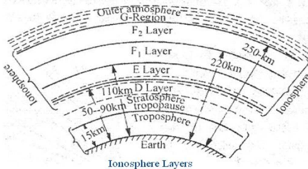
Figure 3 : Structured layers of the ionosphere
