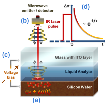
Figure 1. Basic physical principles used in the optoelectronic tongue: (a) generation of free electron–hole pairs near the silicon surface under absorption of IR laser pulse; (b) dependence of microwave reflectivity on concentration of the free charge carriers; (c) modulation of surface band bending by analyte–silicon interaction and applied voltage bias; (d) time-resolved photoconductivity decay due to recombination of the generated electron–hole pairs as a function of surface band bending.
