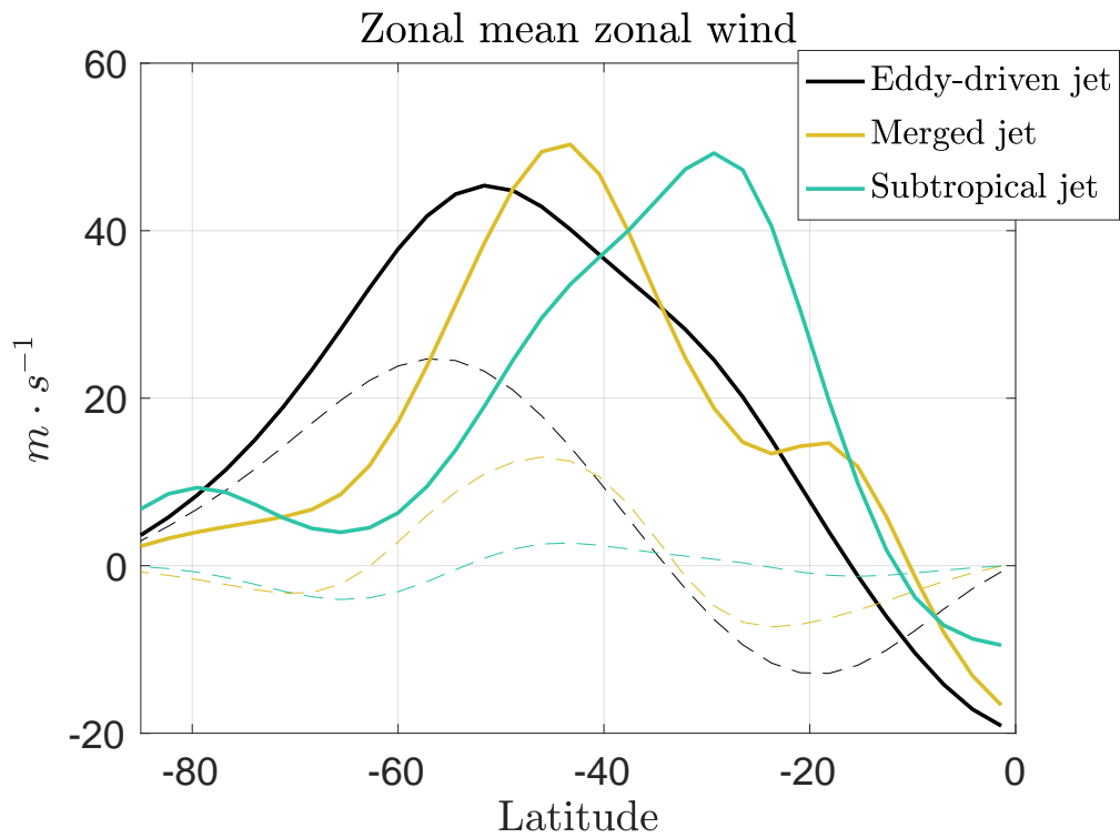
Figure A1. zonal-mean zonal wind ( m s^{-1} ) in the upper ( \bar{u}_u , thick solid lines) and lower ( \bar{u}_l , thin dashed lines) layers of the 2-layer QG model, for simulation number 1 from the eddy-driven jet regime, simulation number 20 from the merged jet regime and simulation number 27 from the subtropical jet regime. Colours indicate the different jet regimes as in the legend. See Table A1 for the parameters of the simulations.
