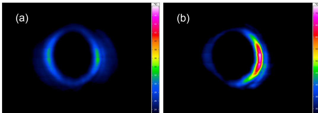
Figure 9. THz far-field beam patterns registered (a) at almost zero mutual FH and SH beam displacement and tilt and (b) for the beam displacement of about 40 \mu\text{m} and tilt of about -0.7 \text{ mrad} .
