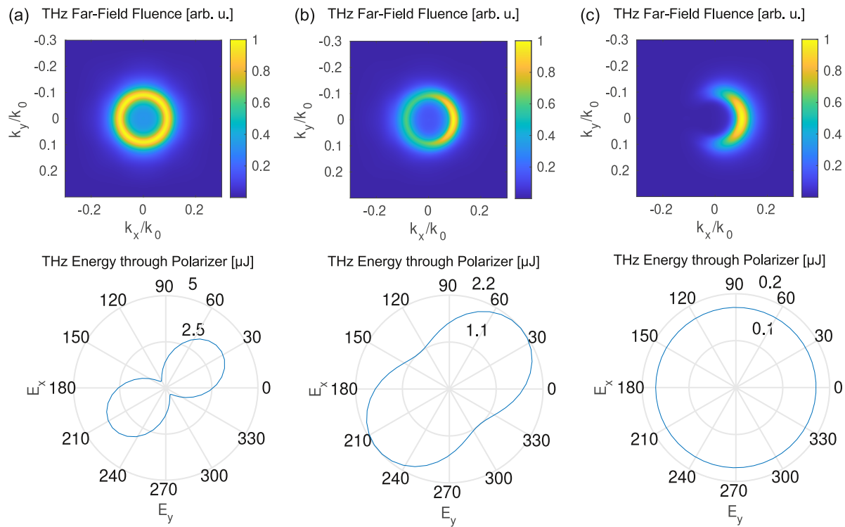
Figure 11. CP-S THz far-field fluence ( \nu < 90 THz). (a) Perfect beam alignment. (b) SH beam displacement of about 4 \mu\text{m} and tilt of about -0.04 mrad. (c) SH beam displacement of about 40 \mu\text{m} and tilt of about -0.4 mrad.
