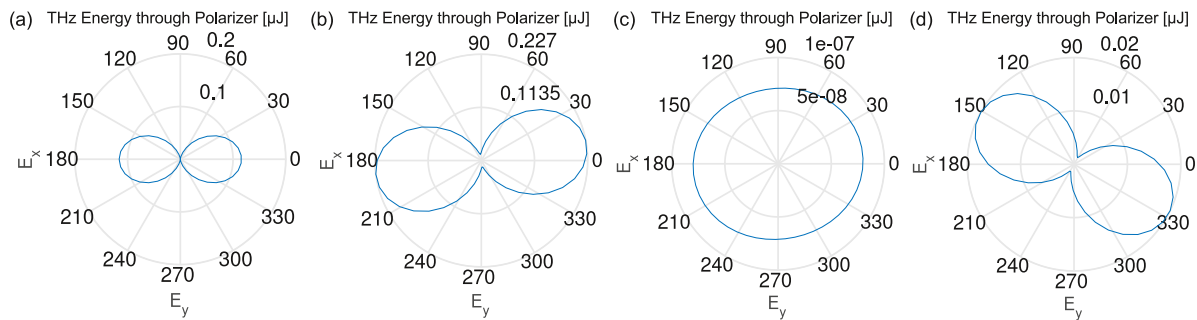
Figure 6. THz transmitted energy through a polarizer obtained at z = 500 \mu\text{m} from 3D UPPE simulations of two-color Gaussian beams in an argon gas jet for different polarization states: (a) LP-P, (b) CP-S, (c) CP-C, and (d) an elliptically-polarized pulse close to CP-C configuration with an ellipse ratio decreased by 10 % and \theta = -0.446\pi . The numbers refer to iso-contour energy levels.
