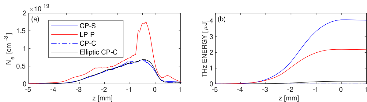
Figure 10. 3D UPPE simulations of two-color Gaussian beams corresponding to the above experiments in air (Fig. 8) for different polarization states: LP-P (red solid curve), CP-S (blue solid curve), and CP-C (dash-dotted blue curve). The black curve refers to an elliptically-polarized pulse close to a CP-C pump with \rho = 0.9 and \theta = -0.446\pi . (a) Peak electron density and (b) corresponding THz energy yields along the propagation axis. Note that the electron density triggered by CP-S and CP-C pulses almost overlap while the CP-C pulse-driven THz energy is close to zero.
