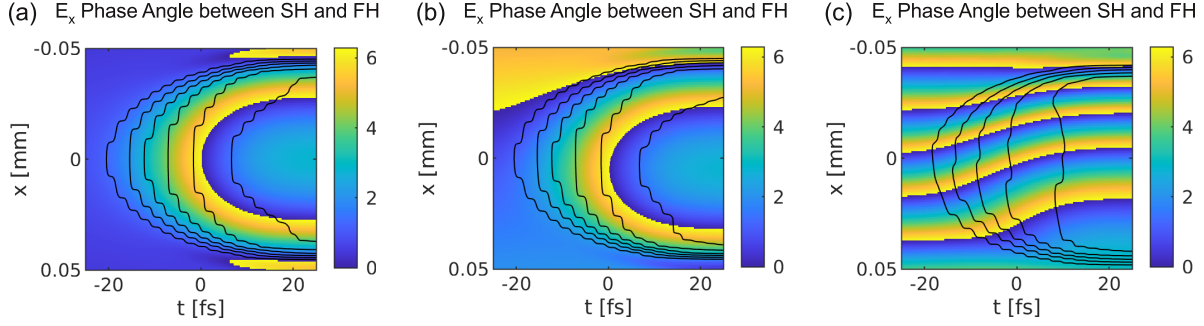
Figure 12. Phase angle between E_x^{\text{SH}} and E_x^{\text{FH}} [ \arg(E_x^{\text{SH}}) - 2\arg(E_x^{\text{FH}}) ] for CP-S pump pulses in the y = 0 plane, 2 mm before the geometrical focus for (a) perfect beam alignment, (b) beam displacement of about 4 \mu\text{m} and tilt of about -0.04 \text{ mrad} , and (c) beam displacement of about 40 \mu\text{m} and tilt of about -0.4 \text{ mrad} . The black lines show iso-electron density surfaces.
