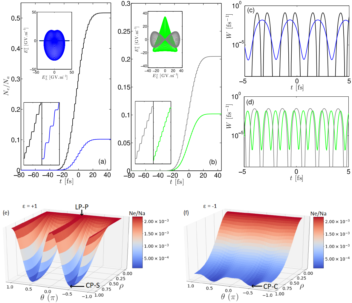
Figure 1. (a,b) Electron density N_e(t) developed along the laser temporal profile in (a) the LP-P (black) and CP-S cases (blue curves), and (b) the CP-C (green) and LP-O cases (gray curves) for two-color, 60-fs Gaussian pulses with 800-nm FH and 200 TW/cm 2 intensity ionizing argon at ambient pressure. Top insets detail the field polarization patterns. Bottom insets zoom in the steplike increase in N_e(t) over a 10-fs time window. (c,d) Corresponding QST ionization rates. (e,f) Density maps of maximum ratios N_e/N_a for finite ellipticities \rho_1 = \rho_2 \equiv \rho \leq 1 and \theta_1 = \theta_2 \equiv \theta for two colors with (e) same helicity and (f) opposite helicity.
