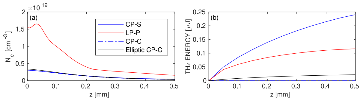
Figure 5. 3D UPPE simulations of two-color Gaussian beams with different polarization states propagating over 500 \mu m in a gas jet configuration (argon) for different polarization states: LP-P (red solid curve), CP-S (blue solid curve), and CP-C pulses with 60-fs FWHM duration (dash-dotted blue curve). The black curve refers to an elliptically-polarized pulse close to a CP-C pump with \rho = 0.9 and \theta = -0.446\pi . (a) Peak electron density and (b) THz energy yields along the propagation axis corresponding to the above plotstyles.
