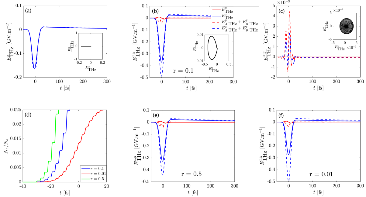
Figure A1. (a,b,c) THz waveforms evaluated semi-analytically (dashed curves) and by the LC model integrated numerically (solid curves) in the three configurations of interest (LP-P, CP-S, CP-C) issued from the pump configurations of Fig. 1 for r = 0.1 . Insets show their corresponding polarization states. (d) Variations in time of N_e/N_a for a CP-S case with different SH intensity fraction r . (e,f) Same curves as in (a-c) for (e) r = 0.5 and (f) r = 0.01 .
