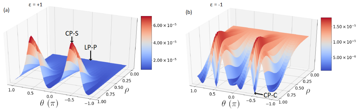
Figure 3. Mapping over (\rho, \theta) of the laser-to-THz conversion efficiency as defined by Eq. (13) from the photocurrents constrained to the same final electron density and for the same pulse and medium parameters as in Fig. 1. (a) \epsilon = +1 , (b) \epsilon = -1 .
