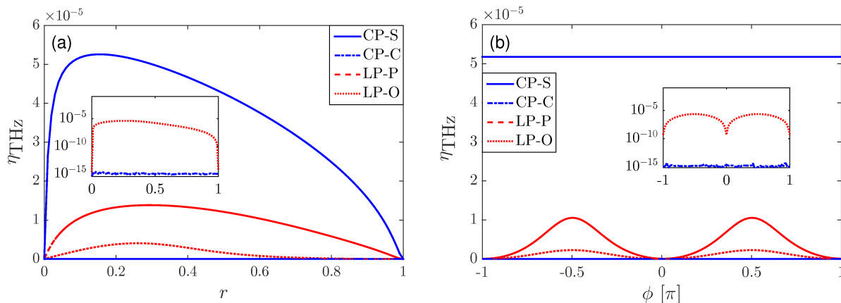
Figure 4. (a) Conversion efficiency using a normalization factor in N_e^{\max} in the cases LP-P, CP-S and CP-C for 60-fs, 200 TW/cm 2 pulses in argon (800-nm FH). (b) Same quantity as a function of the relative phase \phi . Insets zoom in the differences in the THz yields supplied by CP-C and LP-O pulses.
