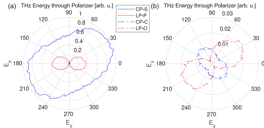
Figure 8. Experimental THz yield versus THz polarizer angle in arbitrary but comparable units. (a) CP-S (solid blue line) and LP-P (solid red line). (b) CP-C (dashed dotted blue line) and LP-O (dashed dotted red line). Energies of the FH and SH pulses were 0.92 and 0.03 mJ, respectively ( r \approx 3.3\% ).
