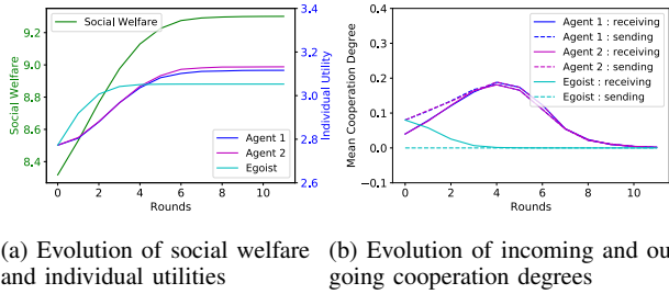
Figure 6: Same simulation as in Fig 5 but with incentive adaptive rate \alpha = 0.3 to prevent exploitation from selfish agent: TFT(\alpha = 0.5, r = 0.2, \alpha = 0.3)
