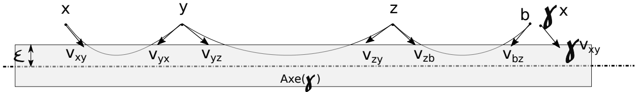
Figure 1 – Broken geodesic close to a hyperbolic axis
