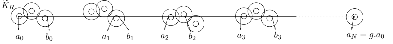
Figure 3 – Long excursions outside \widetilde{K} and \widetilde{K}_R
