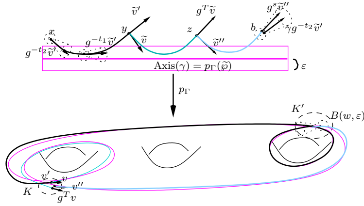
Figure 2.2: Connecting lemma
