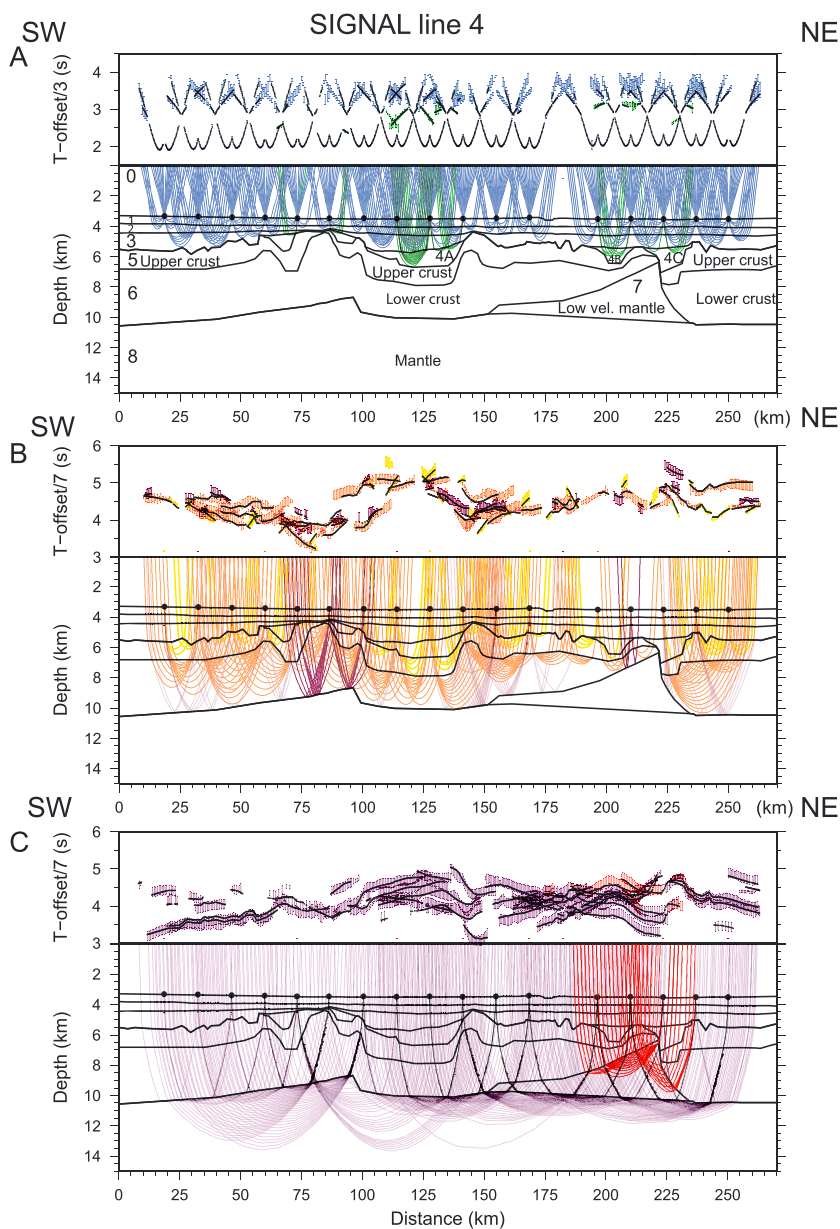
Figure 5. Ray tracing along SIGNAL Line 4. Layers are detailed in the text. (a) The blue rays and traveltimes are direct water waves and sedimentary phases P_{s1} , P_{s2} , and P_{s3} . The green rays and traveltimes correspond to phase P_{s4} in the deep, high-velocity basins associated with layer 4. (b) Yellow rays and traveltimes are related to the P_{c1} phase associated with the upper crustal layer. Orange and purple rays, respectively, correspond to phases P_{c2} (lower crust) and the PmP reflection. (c) Thick red rays turn in layer 7, while purple rays represent the Pn mantle phase. Black lines superimposed on the arrival times and their uncertainties are the calculated traveltimes from the final model (see Figure 9).
