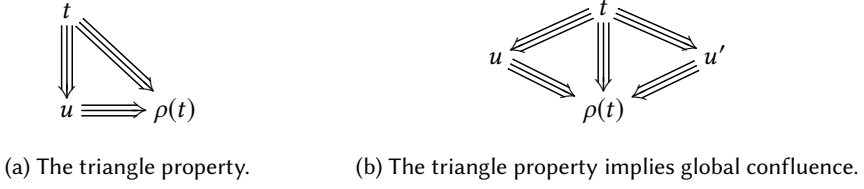
Fig. 1. A visual representation of Definition 4.1 (left) and Lemma 4.2 (right).
