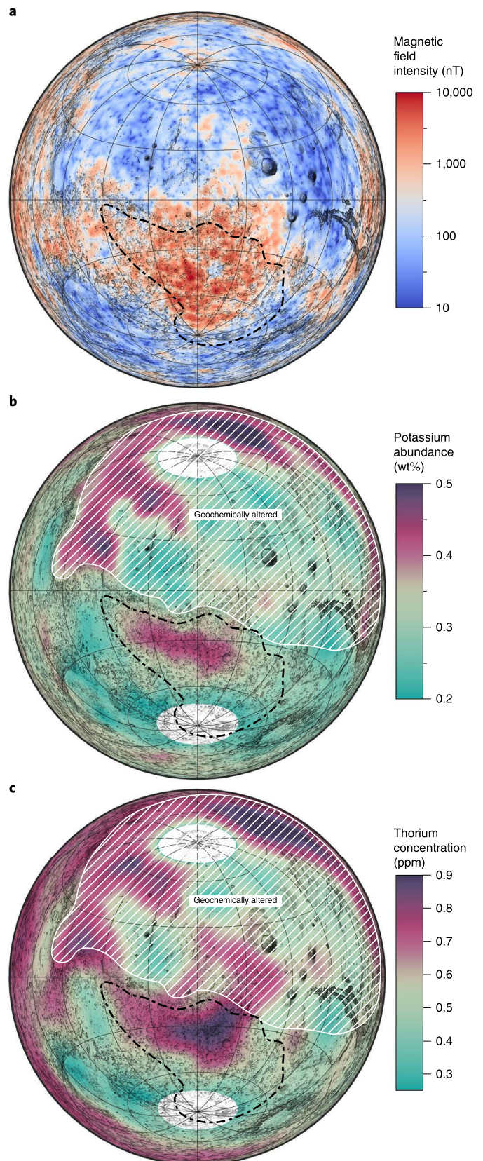
Fig. 4 | The geophysical and geochemical signature of the Cimmeria–Sirenum block. a , The magnetic field intensity, evaluated at the surface of Mars 24 . b , The potassium concentration (wt%) 26 . c , The thorium concentration (ppm) 26 . In b and c , the northern hemisphere is hatched out to focus attention on the signatures south of the dichotomy. The maps are in Lambert azimuthal equal-area projection, centred on 0°, and cover all of Mars except for a small region on the opposite hemisphere. The maps are overlaid on the present-day topography for reference. The Cimmeria–Sirenum crustal block is enclosed by a dash-dot line.
