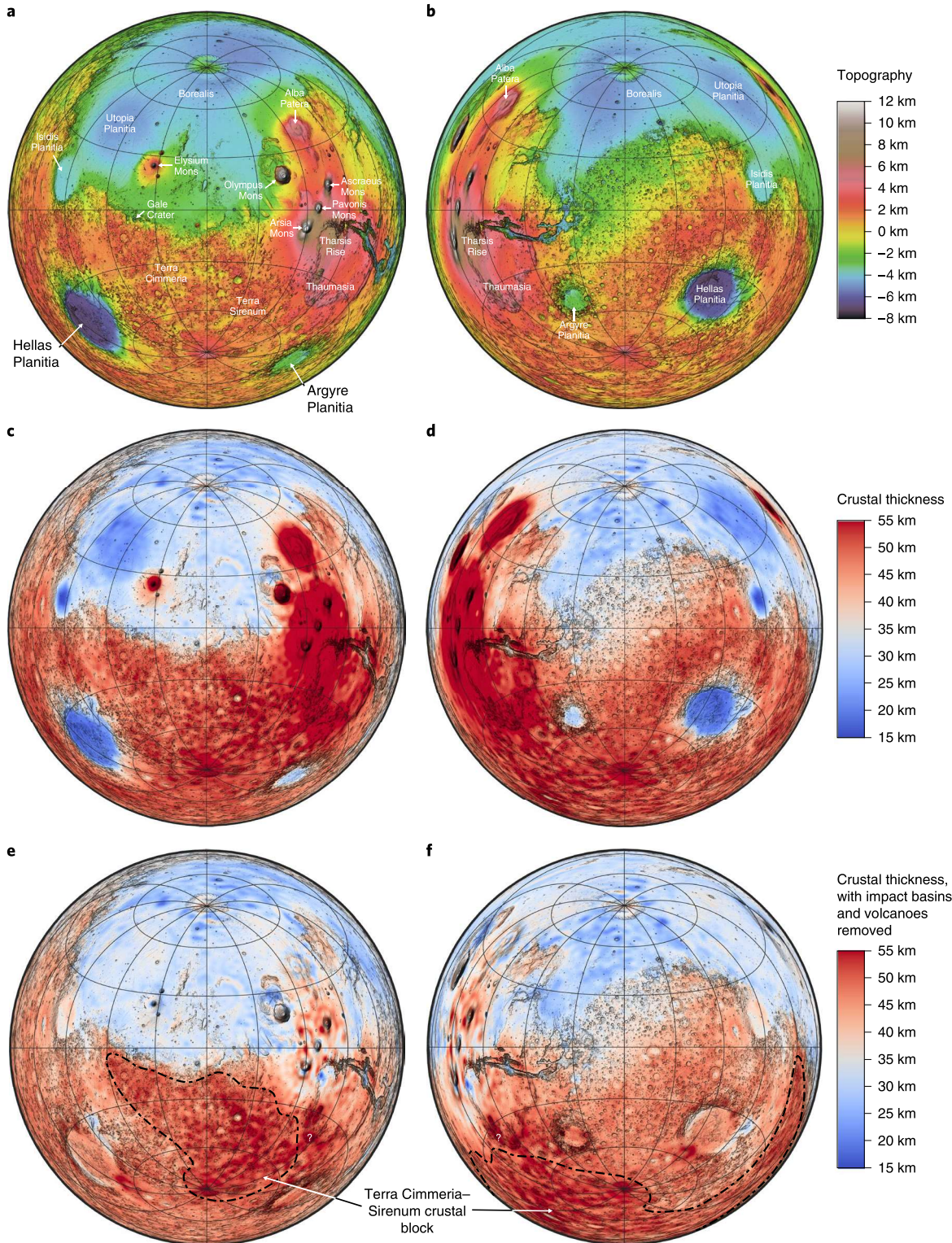
Fig. 1 | A global view of the crustal structure of Mars. a,b , The Mars Orbiter Laser Altimeter topography of Mars with the features of interest labelled 9 . c,d , The crustal thickness of Mars based on crustal model B (ref. 16 , Methods). e,f , The crustal thickness of Mars after removing all of the large impact basins and volcanic features. The Cimmeria-Sirenum crustal block is enclosed by a dash-dot line. The question mark to the east of the block indicates the unclear boundary between the Thaumasia region and the Cimmeria-Sirenum block due to the possible specific origin of Thaumasia 9 . The maps are in Lambert azimuthal equal-area projection, centred on the equator at longitudes 0° (left column) and 180° (right column). Each map covers all of Mars except for a small region antipodal to the map centre. The maps are overlaid on the present-day topography for reference. Grid lines are in increments of 30° of latitude and longitude.
