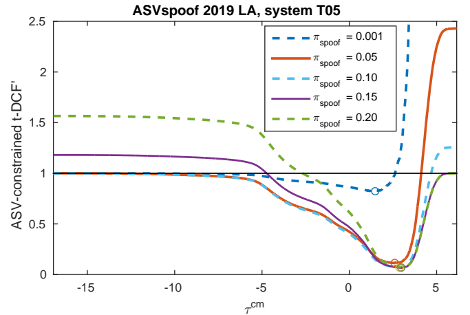
Fig. 7. Normalised ASV-constrained t-DCF w.r.t. the CM threshold for system T45 on ASVspoof 2019 LA.
