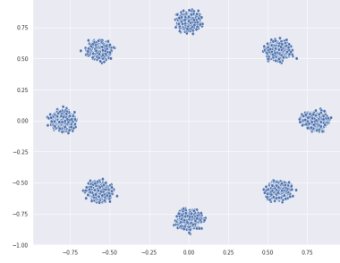
Figure 1: Data distribution x_1, \dots, x_N
