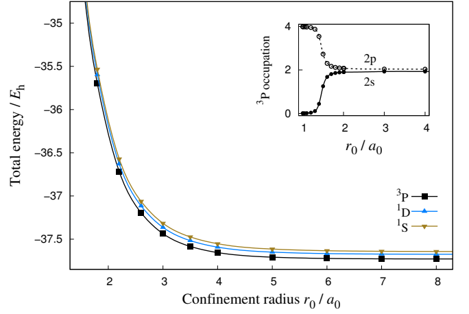
FIG. 15. Energies for the three lowest-lying states of carbon for a stiffness parameter N = 10 using a Gaussian basis. The inset shows the natural occupation numbers of the 2s and 2p shells for the {}^3P state of carbon as a function of the hard-wall confinement radius. The corresponding energies of the hard-wall confined carbon calculated at the CASSCF level are given in the Supplemental Material.
