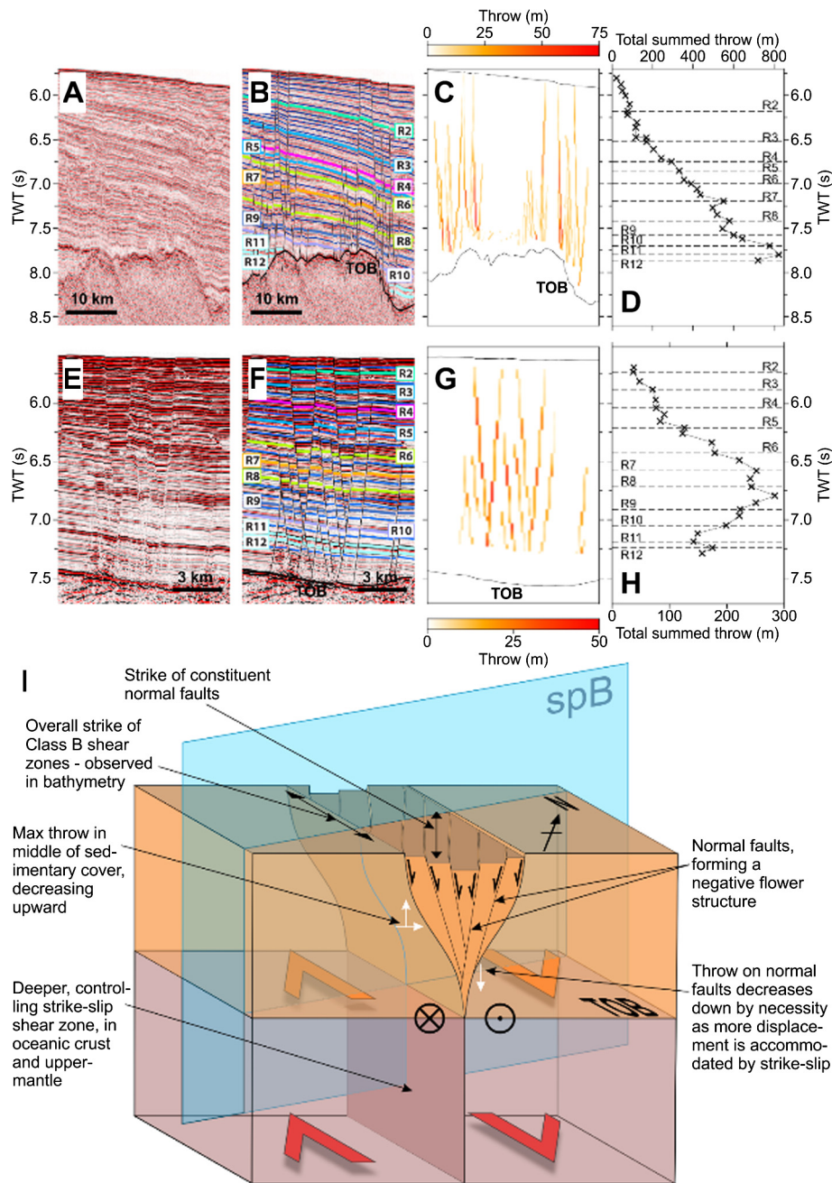
Fig. 6. A-D Example Class C (fracture zone) faulting. (A) uninterpreted and (B) interpreted seismic sections. Note long-wavelength basement topography. (C) Heat map of fault throw, warmer colours indicate greater amounts of throw (see text for method explanation). (D) Fault throw summed across the whole fault zone against depth in two-way-travel-time (also plotted as example F7N in Fig. 7B). (E-H) The same analysis but for Class B faulting. Panel D also plotted as example prof. B in Fig. 7A. In (B and F) subhorizontal coloured lines are used to create plots C and D, and G and H, respectively (where brightly coloured lines are reflectors R1-12, and dull blue lines are additional reflectors interpreted for detailed analysis). TOB – Top of Oceanic Basement. (I) Schematic interpretation of Class B faulting. A purely strike-slip shear fault at depth, within the crust and upper mantle creates extension in the sedimentary cover (see text). spB – Seismic Profile B.
