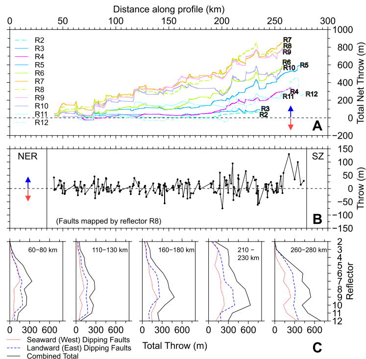
Fig. 9. Along-profile B analysis. (A) Differential cumulative throw from west to east for reflector R1-12 as a function of the differential between E- and W-dipping faults, with E-dipping faults assigned positive values (towards the subduction zone) and W-dipping faults assigned negative values (towards the NER), indicating a dominance of E-dipping faults. Red arrow indicates W-dipping faults dominant, blue arrow indicates E-dipping faults dominant. (B). Along profile throw of reflector R8 (~7 Ma) for individual faults (arrows and +ve/-ve values assigned as in (A)). (C) Displacement with depth profiles for a set of example 20 km along-profile segments (from seismic profile B) where throw is summed for all faults within the segment. Results show changing depth and magnitude of maximum displacement along the profile.
