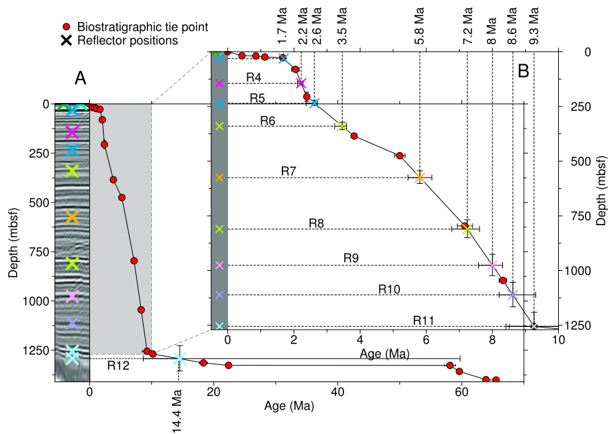
Fig. 3. Interpolation of reflector ages from core-seismic integration. Coloured crosses are seismic reflectors (Fig. 2). The age of reflectors is estimated by time-depth conversion and linear sedimentation accumulation rates between biostratigraphic tie points (McNeill et al., 2017a, 2017b). Errors of reflector ages are \pm 5\% due to velocity uncertainty and the age ranges of tie points.
