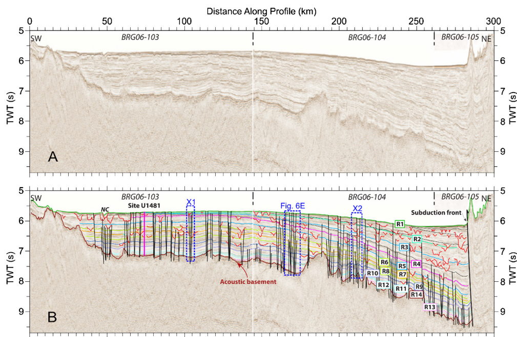
Fig. 2. Regional seismic profile B and position of IODP Site U1481 (vertical pink line). (A) Uninterpreted and (B) interpreted, with faults (black), horizons/reflectors (coloured) R1 to R14 and channels (red). Dashed blue boxes indicate the locations of expanded sections (Fig. 6E (see below) and examples X1 and X2 (see supplementary material). NC = Nicobar Channel; NE = Ninety East Ridge. Fig. 9 shows along profile analysis for this profile.
