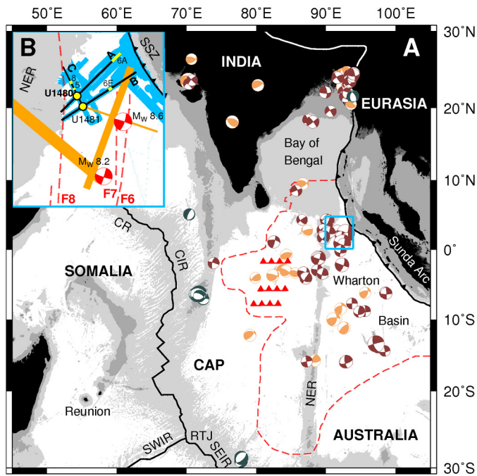
Fig. 1. A) Map showing regional tectonic configuration. Red dashed line indicates extent of diffuse deformation (Gordon et al., 1998). Red toothed lines show schematically the area affected by prominent reverse faults (Bull and Scrutton, 1992; Deplus, 2001). Earthquake focal mechanisms within >2 degrees of narrow plate boundaries, scaled based on magnitude: brown = strike-slip; orange = thrust; blue-grey = normal (Gordon and Houseman, 2015, events 5.3 < M_w < 8.6 , 1976–2014). Light blue box shows enlarged in part B (and approximate area shown in Fig. 10). NER – Ninety East Ridge; CR – Carlsberg Ridge; CIR – Central Indian Ridge; SWIR – South West Indian Ridge; RTJ – Rodriguez Triple Junction; SEIR – South East Indian Ridge; CAP – Capricorn plate. Bathymetry contoured at 2000 m intervals. B). Yellow dots indicate IODP drill sites. Black lines are multichannel seismic profiles A–C, sections highlighted in yellow indicate the locations of seismic data depicted in Figs. 5, 6 and 8. Light blue shaded area shows multibeam bathymetry coverage used in this study (presented in Fig. 4) Red, dashed lines are fracture zones (Jacob et al., 2014) (nomenclature from Singh et al., 2011). Focal mechanisms for April 2012 events in red, data from Global centroid moment tensor project [www.globalcmt.org]. Orange shaded area shows rupture plane model for 2012 earthquakes from Wei et al. (2013). SSZ – Sumatra Subduction Zone.
