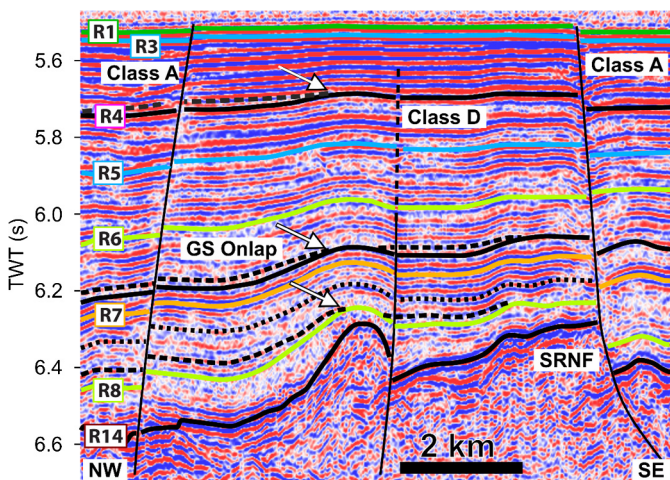
Fig. 8. Example Class D reverse fault structure on NW-SE trending profile C. Additional dashed horizons show onlap of growth strata (GS) onto the crest of the fault-propagation fold (indicated by arrows). Also shown is a spreading-ridge-normal-fault (SRNF) that has been re-activated through Class A strike-slip faulting.
