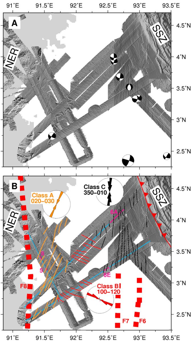
Fig. 4. Distribution of seafloor faulting interpreted from multibeam bathymetry. A) uninterpreted slope map of multibeam data showing intraplate earthquake focal mechanisms (as shown in Fig. 1). B) Interpreted lineations for each fault class (colour coded) and corresponding rose diagrams. Thick red dotted lines represent fracture zones (nomenclature from Singh et al., 2011). Light blue lines indicate seismic profiles and the positions of Figs. 5, 6 and 8 are highlighted in pink.
