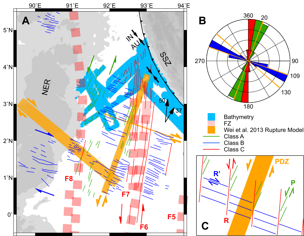
Fig. 10. (A) Compiled fault map of the northern Wharton Basin (from this study; Sager et al., 2013; Hananto et al., 2018). Light blue area shows location of bathymetry data used in this study. Pink areas indicate locations of major Wharton Ridge fracture zones (Singh et al., 2011). Orange areas indicate 2012 earthquakes rupture planes (Wei et al., 2013). Faults are: Class A faults and equivalents (green); Class B faults and equivalents (blue); Class C faults and equivalents (red). Green, blue and red arrows indicate sense of displacement on correspondingly coloured faults. Opposing black arrows (IN-AU) indicate principal deviatoric stress (Gordon and Houseman, 2015). Numbered black arrows are plate motion vectors (McNeill and Henstock, 2014) mm/year. (B) Rose diagram showing average fault class orientations and orientations of the rupture planes for the 2012 earthquakes. (C) Schematic of proposed relationship between these fault sets, as Riedel shears forming in response to a NNE-trending principal displacement zone. NER – Ninety East Ridge, SSZ – Sunda Subduction Zone.
