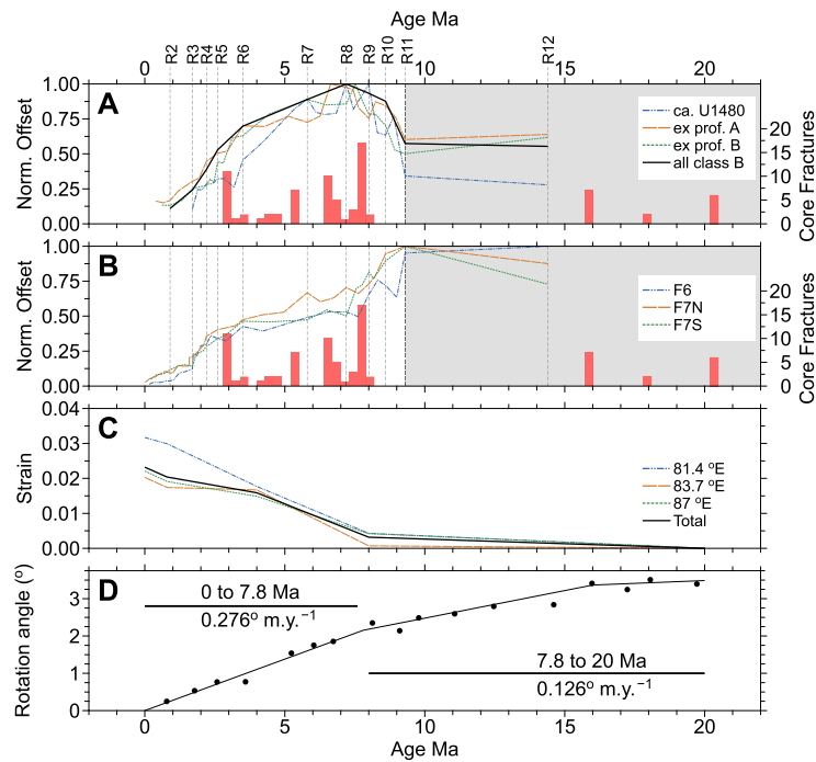
Fig. 7. Examples of fault displacement profiles for different fault classes plotted with depth/sediment age alongside strain of faults west of the NER and plate motion history through time. (A) Class B fault displacement with depth/reflector age. Coloured lines are three fault examples; black line is overall average for all Class B faults. (B) Displacement profiles with depth/reflector age for major fracture zones F6 and F7 (the latter from profile A (F7N) and B (F7S)). The frequency of fractures detecting in core at site U1480 is adjusted to age and superimposed on both (A) and (B). (C) Analysis by Krishna et al. (2009) for strain budget for faults west of the NER from fault throw, plotted against age. Strain is normalized by deformation extent on each seismic profile used (longitude of N-S profiles indicated). (D) India-Capricorn finite rotation angles with time from plate kinematic reconstructions (Bull et al., 2010), showing acceleration around 8 Ma. Used here as a proxy for India-Australia relative motion.
