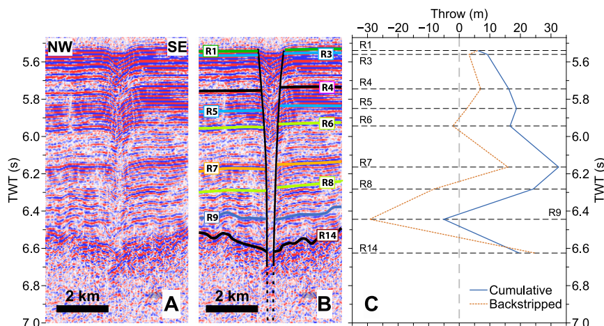
Fig. 5. Example Class A fault on NW-SE trending seismic profile C, (A) uninterpreted and (B) interpreted. Note V-shape of reflectors at the position of the fault and apparent layer thickness changes across the fault. (C) displacement analysis of example fault. Cumulative line shows the total net vertical displacement accumulated by each horizon since deposition, backstripped line indicates how vertical displacement has accumulated with time i.e. how much displacement occurred ca the time of deposition of each horizon. Vertical separation attributed positive values for normal and negative for reverse assuming that the footwall is to the SE.
