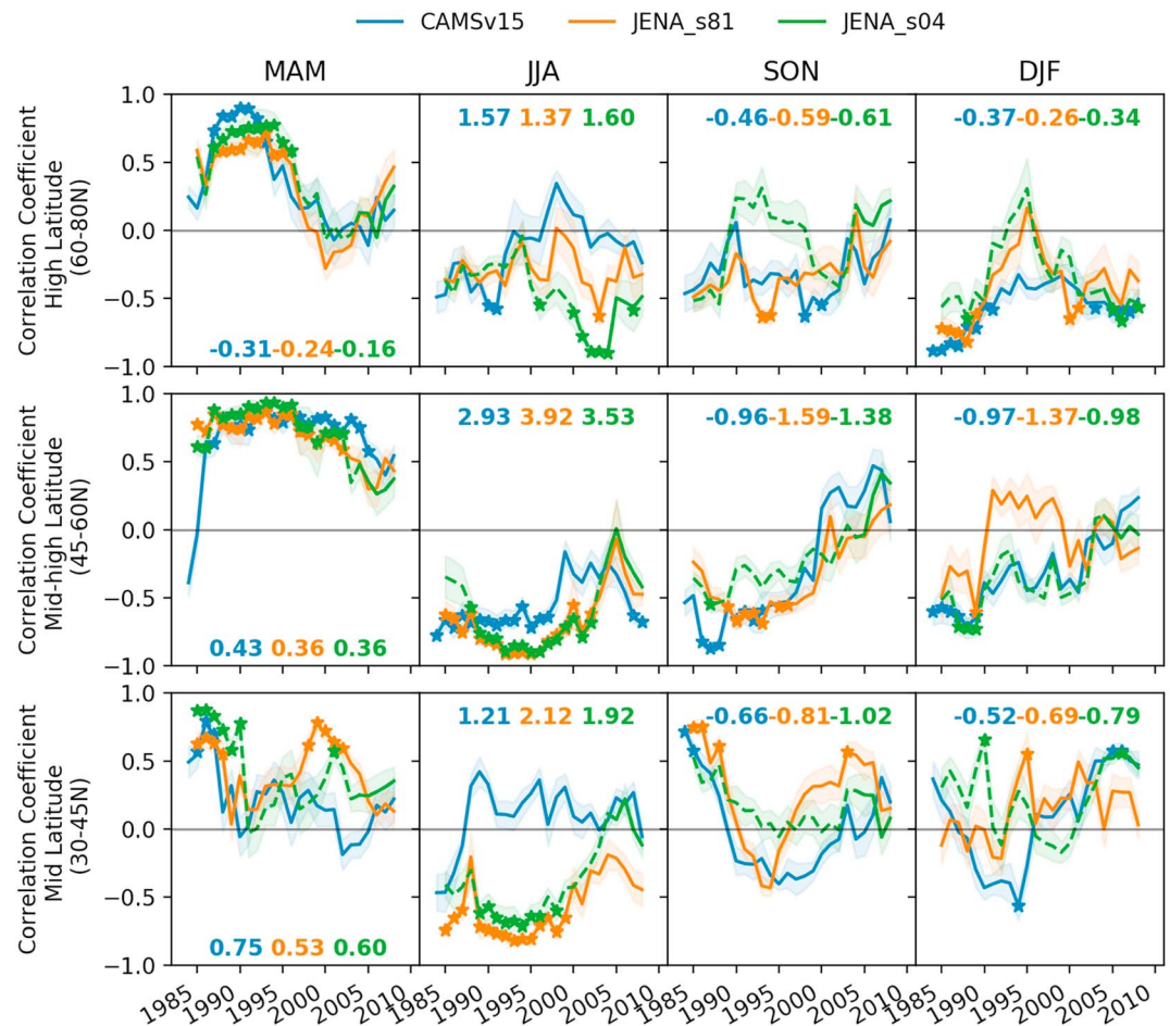
Figure 3. Moving correlations between \Delta NBP and \Delta T using a 10-year window. Each row presents a zonal band (midlatitude, mid-to-high latitude, and high latitude) and each column a season from spring (March–May) to winter (December–February). Both variables are detrended within the moving window, and each data point is drawn at the middle of the analyzing window. The color codes represent the three atmospheric inversions, and the shaded areas show the uncertainty of the correlation coefficients estimated using a bootstrap method; the stars mark significant correlations at the 90% confidence level. The numbers denote the multiyear average net biome productivity (NBP) estimated by the corresponding inversion product with the same color code (a positive NBP value means net land carbon uptake, a negative value means net carbon release from the land to the atmosphere). Note that for the JENA_s04 inversion, results outside its validity period 2004–2015, which does not have consistent network constraint, are shown in dashed lines.
