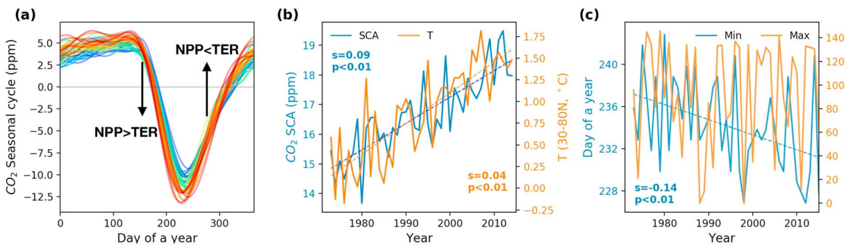
Figure 1. CO 2 seasonal cycles observed at Barrow. (a) Annual CO 2 seasonal cycles from 1971 to 2015 (color codes from blue to red). The comparison of the magnitudes of net primary productivity (NPP) and terrestrial ecosystem respiration (TER) are noted for illustrating their impacts on the CO 2 seasonal cycle. (b) Times series of the SCA (in blue) and the mean annual air temperature (in orange) in the 30–80°N zone. (c) Time series of the dates when CO 2 reaches its seasonal minimum (in blue) and maximum (in orange). The s means the slope of the regression line, and p means the p -value of the linear regression.
