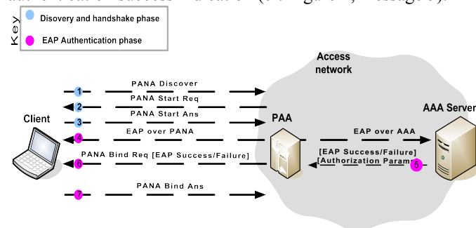
Figure 1. Authentication and Authorization Procedure
