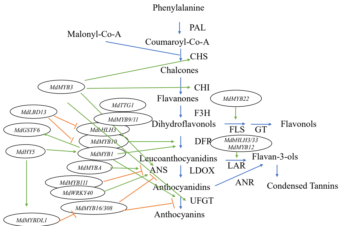
Figure 2. Diagrammatic representation of the anthocyanin biosynthetic pathway and the related TFs in apples. Green arrows indicate TFs activating enzymes in the pathway, while orange barred lines signify a TF inhibiting enzyme expression in the pathway.
