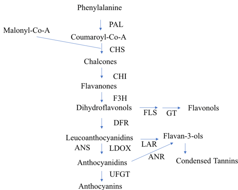
Figure 1. Diagrammatic representation of the flavonoid biosynthetic pathway in apples, according to Takos et al. [14]. PAL, Phe ammonia lyase; CHS, Chalcone synthase; CHI, chalcone isomerase; F3H, flavanone-3 b-hydroxylase; DFR, dihydroflavonol-4-reductase; LDOX, leucoanthocyanidin dioxygenase. UFGT, UDP-glycose: flavonoid-3-O-glycosyltransferase; FLS, flavonol synthase; GT, glycosyl transferase; LAR, leucoanthocyanidin reductase; ANR, anthocyanidin reductase.
