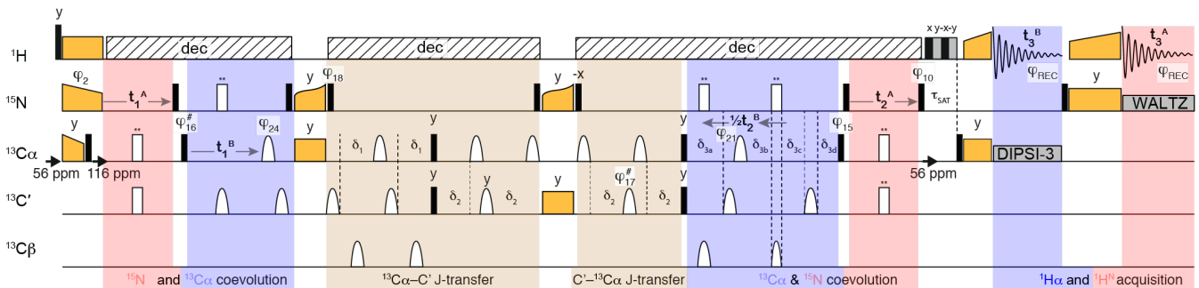
Figure S5. Radiofrequency (RF) pulse scheme for the “8-in-1” experiment. Heteronuclear cross-polarization (CP) transfers are shown as either wide rectangular, trapezoid or tangential orange shapes simultaneously on two or three RF channels. RF strength, duration and detailed shapes for CP transfers are provided in Table S2. Solid and open pulses represent high-power 90^\circ and 180^\circ pulses, respectively. Open pulses marked with double star (**) denote composite 180^\circ pulses 90_x^\circ 180_y^\circ 90_x^\circ , which were used to minimize signal losses on the pathways other than the decoupled one. In our implementation (see Section J) these pulses are optional, and can be skipped for short evolution times. Open bell shapes on ^{13}\text{C} channels represent \text{Q3}^3 (for ^{13}\text{C}\alpha and ^{13}\text{C}' ) and \text{ReBURP}^4 (for ^{13}\text{C}\beta ) selective pulses. Pulse durations and peak RF strength were 161.5, 178.5 and 960.9 \mu\text{s} and 20.43, 18.49 and 6.52 kHz for ^{13}\text{C}\alpha , ^{13}\text{C}' and ^{13}\text{C}\beta pulses respectively. Note that the moderately selective ^{13}\text{C}\alpha pulses affect both ^{13}\text{C}\alpha and ^{13}\text{C}\beta spins. Heteronuclear ^1\text{H} decoupling during indirect evolution or J -transfer periods is shown in hatched grey. Swept-TPPM 5-6 ^1\text{H} decoupling with RF field of 10 kHz and pulse length of 25 \mu\text{s} was used. WALTZ-16 7 and DISPI-3 8 with RF strength of 10 and 20 kHz, and pulse lengths of 25 and 12.5 \mu\text{s} , were used for ^{15}\text{N} and ^{13}\text{C} decoupling during signal acquisition, respectively. The MISSISSIPPI water suppression, 9 with duration \tau_{\text{SAT}} of 200 ms and RF strength of 25.4 kHz, is shown as a composite block of four solid and grey pulses. Relaxation-optimized ^{13}\text{C}\alpha - ^{13}\text{C}' J -transfer delays \delta_1 and \delta_2 were 4.2 and 4.3 ms, respectively. They were derived from the formula: \delta = \frac{1}{2} \tan^{-1}(\pi J T_2') / (\pi J) , where T_2' denotes either the ^{13}\text{C}\alpha or \text{C}' refocused coherence lifetime (estimated to 48 and 70 ms, respectively). ^{13}\text{C}\alpha - ^{13}\text{C}' J -coupling constant of 55 Hz was assumed. ^{13}\text{C}\alpha evolution in t_2 (denoted t_{2B} ) was performed in constant- or real-time, depending on whether t_{2B} exceeded the relaxation-optimized transfer delay \delta_1 or the maximum transfer time \delta^* = \frac{1}{2} (2J)^{-1} . Namely, the delays \delta_{3a} , \delta_{3b} , \delta_{3c} , \delta_{3d} were set to respectively \delta_1 - \frac{1}{2} t_{2B} , \frac{1}{4} t_{2B} + \frac{1}{2} (\delta_1 - pw^{\text{CB}}) , \frac{1}{4} t_{2B} + \frac{1}{2} (\delta_1 - pw^{\text{CB}}) and 0 if t_{2B} < 2(\delta_1 - pw^{\text{CB}}) ; to respectively pw^{\text{CB}} , \frac{1}{2} t_{2B} , \frac{1}{2} t_{2B} and 0 if 2(\delta_1 - pw^{\text{CB}}) \leq t_{2B} < 2(\delta^* - pw^{\text{CB}}) ; and to respectively pw^{\text{CB}} , \frac{1}{2} t_{2B} , \delta^* - pw^{\text{CB}} and \frac{1}{2} t_{2B} - (\delta^* - pw^{\text{CB}}) for t_{2B} \geq 2(\delta^* - pw^{\text{CB}}) , where pw^{\text{CB}} stands for the duration of ^{13}\text{C}\beta -selective pulse. All pulses have phase x unless indicated. The phase cycle was (for convenience the numbering of phases is consistent with pulse sequence code provided below): \phi_2 = \{y, -y\} , \phi_{10} = \{x, x, -x, -x\} , \phi_{15} = \{x, x, -x, -x\} , \phi_{16} = \{x, -x\} , \phi_{17} = y , \phi_{18} = x , \phi_{21} = x , \phi_{24} = x , and \phi_{\text{rec}} = \{y, -y, -y, y\} . Quadrature detection in the indirect dimensions was accomplished using the States-TPPI 10 method by incrementing \phi_2 and \phi_{16} (in t_1 ) and decrementing \phi_{10} and \phi_{15} (in t_2 ), independently from t_1 and t_2 time incrementation. Additionally, a quarter spectral window upfield and downfield shift for respectively ^{15}\text{N} and ^{13}\text{C}\alpha resonances, was implemented by incrementing \phi_2 and \phi_{16} in synchrony with t_1 time incrementation, i.e. \phi_2 = \{y, -y\} + 90^\circ \times ((t_1 sw_1) \bmod 4) . The ^{15}\text{N} offset was set to 117.5 ppm while the ^1\text{H} offset was set on resonance with the \text{H}_2\text{O} line (approx. 4.8 ppm). The ^{13}\text{C} offset was set to the center of the ^{13}\text{C}\alpha band (56.4 ppm) for the first and last CP transfer, and in-between the ^{13}\text{C}\alpha and ^{13}\text{C}' regions (116.4 ppm) for the rest of the sequence (as indicated by horizontal arrows). Effectively, both t_1 and t_2 ^{13}\text{C}\alpha evolution is performed off-resonance, and the extra acquired phase is compensated by the time-proportional phase incrementation on refocusing pulses with phases \phi_{21} and \phi_{24} : \phi_{21} = \{x\} + 180^\circ \Delta\Omega \cdot t_2 , \phi_{24} = \{x\} + 180^\circ \Delta\Omega \cdot t_1 (in degrees), where \Delta\Omega = \Omega_{\text{C}\alpha} - \Omega_0 (in hertz). Also, all shaped ^{13}\text{C} pulses are performed off-resonance by a stepwise phase modulation with respective offset difference \Omega_{\text{C}\alpha} - \Omega_0 = -60 ppm, \Omega_{\text{C}'} - \Omega_0 = 60 ppm or \Omega_{\text{C}\beta} - \Omega_0 = -91 ppm (where \Omega_0 stands for the carrier offset). The ^{13}\text{C} pulses for ^{15}\text{N} - ^{13}\text{C}\alpha and ^{15}\text{N} - ^{13}\text{C}' CP transfers are performed with relative offsets \Omega_{\text{C}\alpha} - \Omega_0 = -60 ppm = -120 ppm and \Omega_{\text{C}'} - \Omega_0 + 60 ppm = +120 ppm, respectively. The additional \pm 60 ppm offset is to minimize undesired ^{15}\text{N} - ^{13}\text{C}' and ^{15}\text{N} - ^{13}\text{C}\alpha transfers during these CP transfers (these lossy transfers arise due to the direction of the ^{15}\text{N} ramp enforced by other pathways). Zero phase alignment for the ^{13}\text{C} pulses during ^{15}\text{N} - ^{13}\text{C}\alpha and ^{15}\text{N} - ^{13}\text{C}' CP transfers was enforced at the end and the beginning of the pulse, respectively. While this ensures the phase agreement for ^{13}\text{C} pulses between these two CP transfers, a constant phase difference with respect to the 90^\circ pulse before ^{15}\text{N} - ^{13}\text{C}\alpha CP (causing a zero-order phase for ^{13}\text{C}\alpha in \omega_1 ), and with respect to the 90^\circ pulse after ^{15}\text{N} - ^{13}\text{C}' CP is generated (leading to the loss of signal). It is thus necessary to correct these phase shifts, e.g. by empirically optimizing the phases \phi_{16} and \phi_{17} , while a single pathway is selected (see Section J). In our experiment, the best values of 310^\circ and 75^\circ were found for \phi_{16} and \phi_{17} , respectively. Additionally, as shown in Figure S6, among 8 recorded types of correlations there are four pairs sharing the same frequency regions in \omega_1 , \omega_2 and \omega_3 dimensions (e.g. ^{13}\text{C}\alpha(i-1) - ^{15}\text{N}(i) - ^1\text{H}^{\text{N}}(i) and ^{13}\text{C}\alpha(i) - ^{15}\text{N}(i) - ^1\text{H}^{\text{N}}(i) ). They can be discriminated based on which term, i.e. either ^{15}\text{N} or ^{13}\text{C} , is present between the ^{15}\text{N} - ^{13}\text{C}\alpha and ^{15}\text{N} - ^{13}\text{C}' CP transfers. Here, an extra 180^\circ incrementation of phase \phi_{18} is introduced as the innermost loop, and the interleaved data requires a linear combination (addition and subtraction) during signal processing as described in section E.
