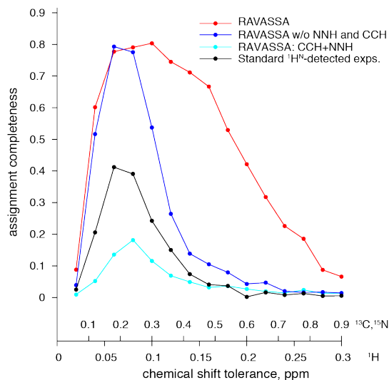
Figure 4. Characterization of the sensitivity of the automated assignment with respect to the matching tolerance. Red, blue, cyan and black dots indicate the assignment completeness, defined as the ratio of strongly assigned to all 1 H N , 1 H \alpha , 13 C \alpha , 13 C \beta and 15 N resonances, obtained with the complete and reduced RAVASSA datasets, as well as with the classical 1 H N detected datasets, 1 respectively. Points are connected for eye guidance only.
