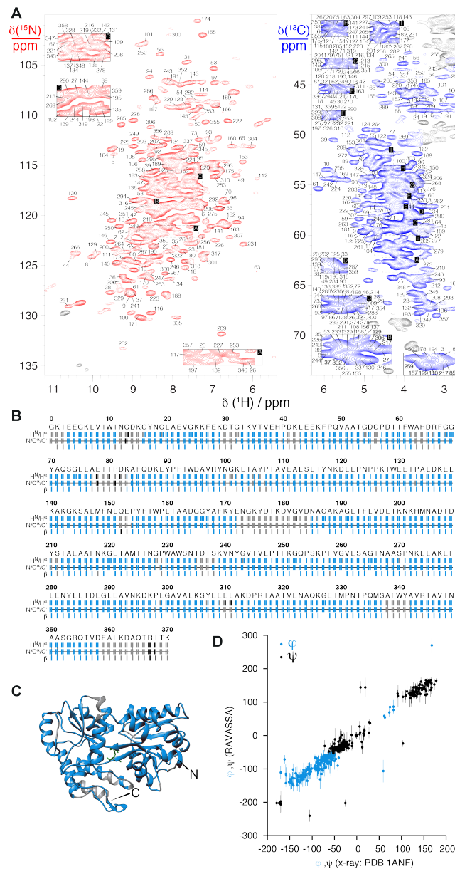
Figure 5. Assigned dipolar heteronuclear correlation spectrum of maltose binding protein: 15 N- 1 H (red contours) and \alpha -region of 13 C- 1 H correlations (blue contours), acquired simultaneously. (B) Result of automated FLYA resonance assignment of MBP. Resonances with “strongly” determined chemical shifts are marked in blue (or in black, if located in isolated short fragments and thus discarded), while those below confidence threshold are shown in grey. (C) X-ray derived structural model of maltose binding protein (PDB 1ANF) with assigned residues marked in blue. (D) Backbone dihedral angles \phi and \psi predicted based on assigned chemical shifts and in the X-ray structure.
