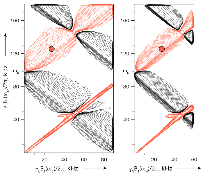
Figure S4. Standard (sequential) CP conditions for ^1\text{H} - ^{13}\text{C} (left) and ^1\text{H} - ^{15}\text{N} CP (right) at 107 kHz MAS in a 0.7 mm Bruker HCN probe on a 800 MHz spectrometer. Signal intensity was evaluated by stepwise variation of ^1\text{H} and either ^{13}\text{C} or ^{15}\text{N} RF strength during a fixed contact time CP following the first ^1\text{H} pulse in a 1D (H)CH or (H)NH experiment (“first FID”). The intensities along detected ^1\text{H} dimension were summed over the aliphatic or amide ^1\text{H} range. Zero-quantum (ZQ) and double-quantum (DQ) CP show opposite signs and are shown in red and black, respectively. Red disks connected by a horizontal dashed line (i.e. at common ^1\text{H} RF strength) indicate the optimal CP conditions for both sequential transfers, which are chosen here for the simultaneous CP (SIM-CP).
