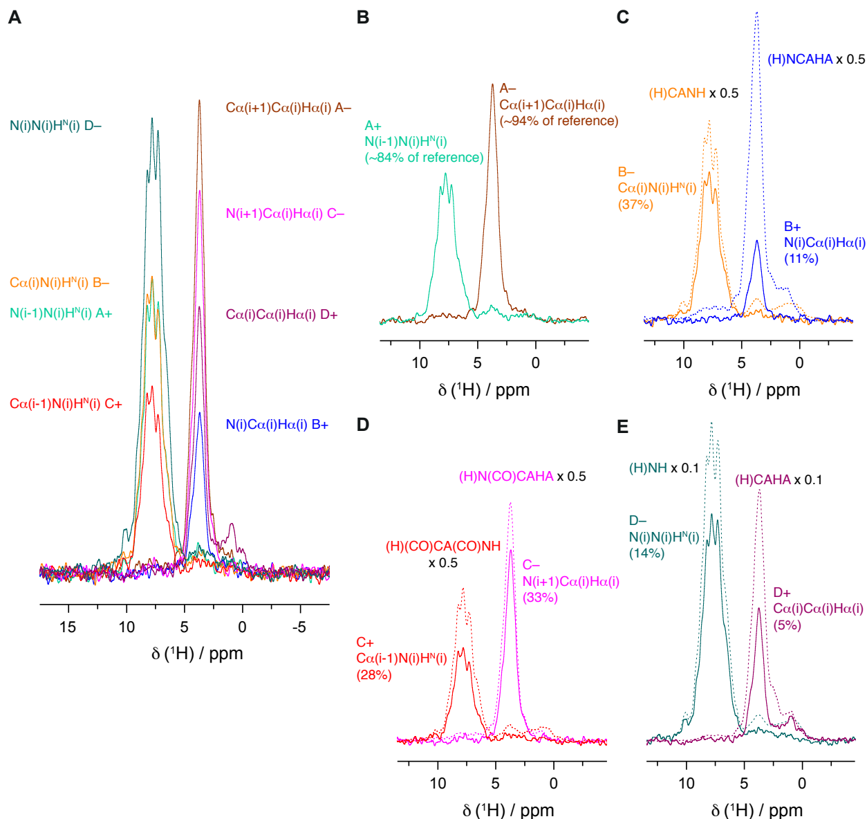
Figure S10. Relative intensities of eight RAVASSA pathways as observed in ^1H 1D first-FID spectra (A), color-coded and labeled “A+”, “A-“ etc. in agreement with pathway description in respective panels A, B, etc. of Figure S6. Selection of pathways was performed using appropriate phase cycling as described in Section J. Note that due to lack of resolution and line width differences, the intensity comparison is valid only between ^1H^N - or ^1H\alpha -detected pathways. Panels B-E show the 1D intensity comparisons of RAVASSA pathways (divided into four classes as in Figure S6) with the corresponding separately optimized serial experiments (dashed curves). Relative integral of respective 1D signals is given for every pathway.
