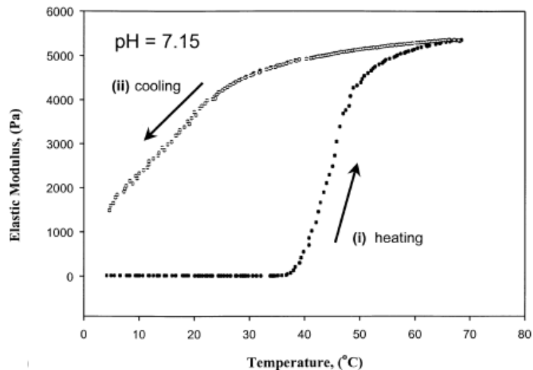
Figure 6. Elastic modulus G' variations of a CS/GP thermosensitive hydrogel as a function of temperature at pH = 7.15 [102]
