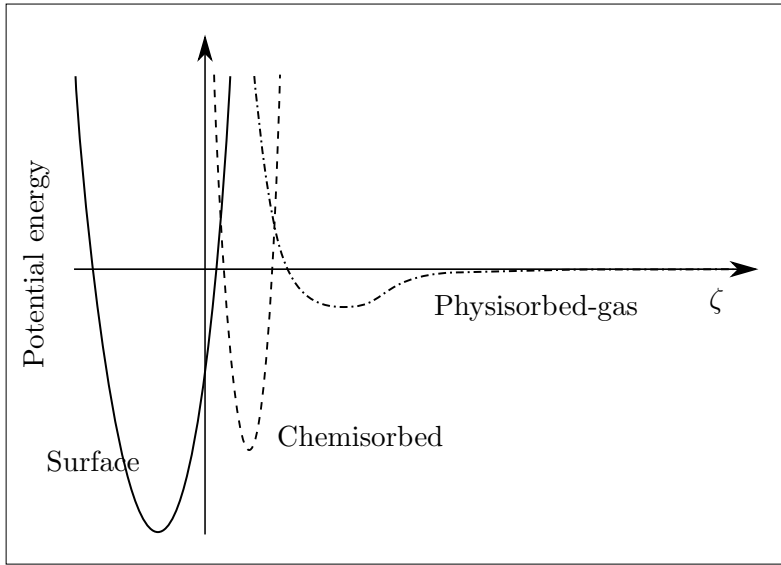
Figure 1: Typical surface interaction potentials as function of the distance from surface in arbitrary units.
