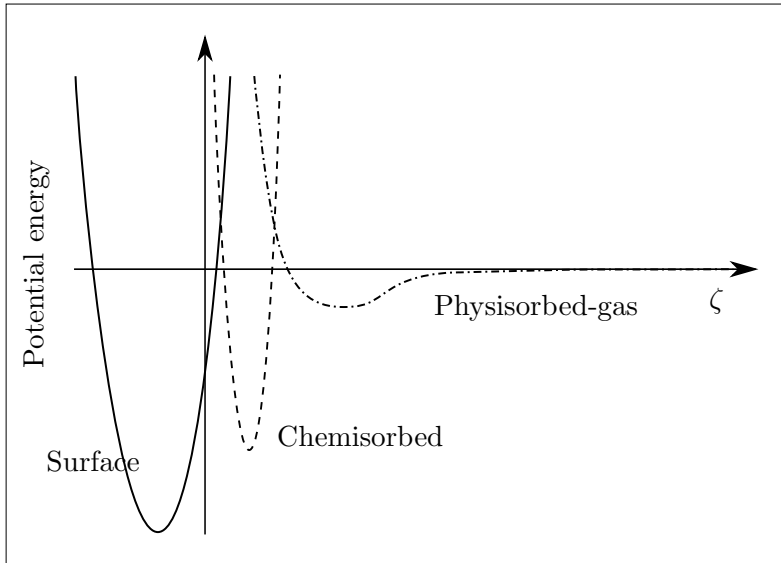
Figure 1: Typical surface interaction potentials as function of the distance from surface in arbitrary units.
