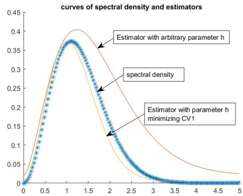
Figure 2. Curves of spractral density, its estimators.
