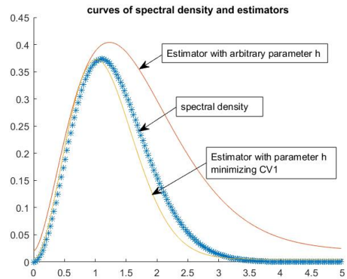
Figure 2. Curves of spectral density, its estimators.
