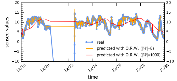
Fig. 5: An extract (Dec. 18, 2019 – Dec. 30, 2019) from the prediction applied during P3 with O.R. and |W|=8 .
