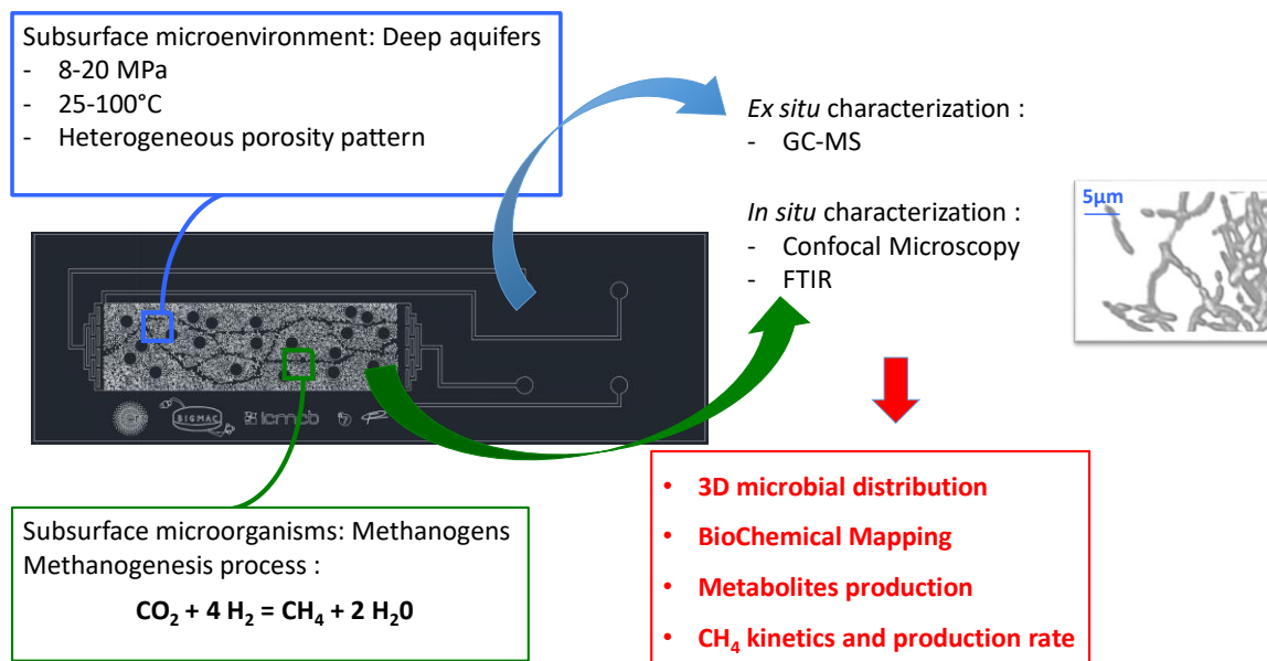
Figure 1. Example of a high pressure geological laboratory on a chip for investigating methanogens subsurface microorganisms for CO 2 bioconversion to methane in deep saline aquifers.
