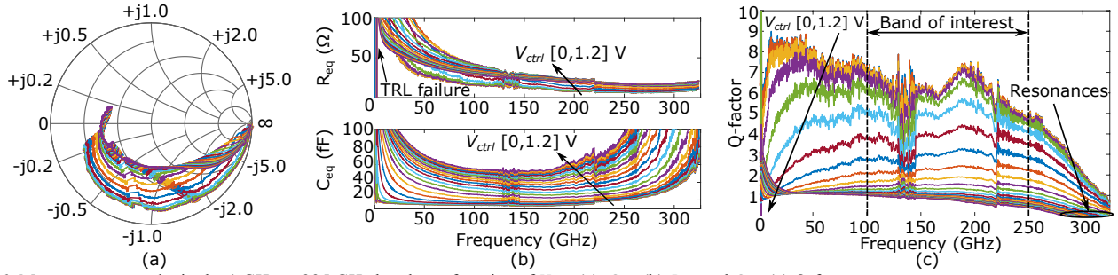
Fig. 6. Measurement results in the 1 GHz to 325 GHz band as a function of V_{ctrl} (a) S_{11} . (b) R_{eq} and C_{eq} . (c) Q-factor.
