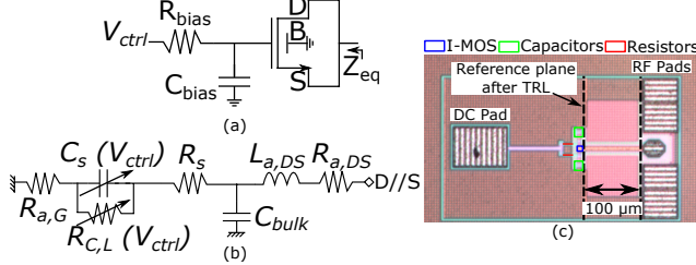
Fig. 5 (a) I-MOS varactor architecture. (b) Proposed small-signal model. (c) Micrograph of the fabricated circuit.
