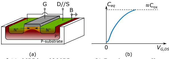
Fig. 2 (a) nMOS-based I-MOS varactor. (b) Capacitance versus V_{G,DS} .
