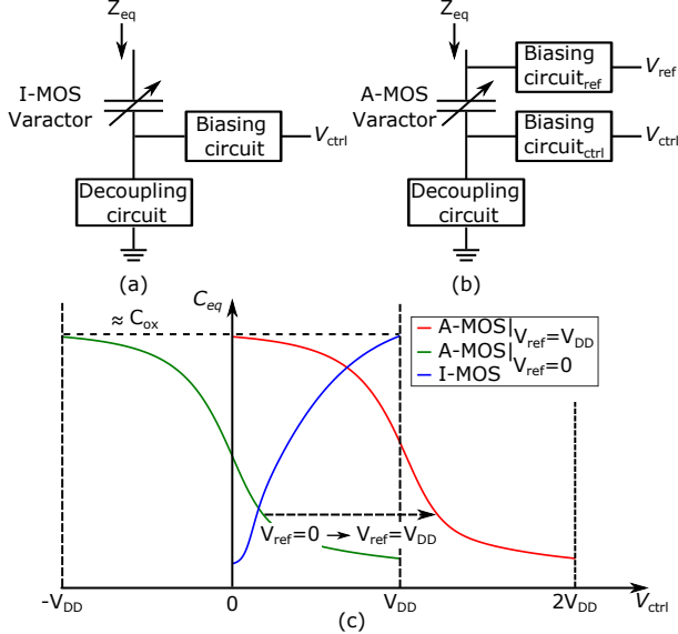
Fig. 3. (a) I-MOS varactor and the biasing/decoupling circuits. (b) A-MOS varactor and the biasing/decoupling circuits. (c) Capacitance versus V_{ctrl} for: (i) a thick-oxide A-MOS varactor with V_{ref} = 0 V (i.e. only Biasing Circuit,ctrl is necessary), (ii) a thick-oxide A-MOS varactor with V_{ref} = V_{DD} and (iii) an I-MOS varactor.
