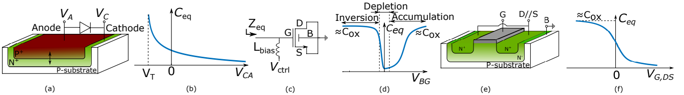
Fig. 1. (a) PN junction and its symbolic representation as a diode. The arrows depict the movement of the charge carriers when the voltage difference between cathode and anode ( V_{CA} ) increases. (b) Capacitance versus V_{CA} . (c) nMOS transistor with B, D and S connected together. (d) Input capacitance versus V_{BG} . (e) A-MOS varactor. (f) Capacitance at D//S level versus V_{G,DS} .
