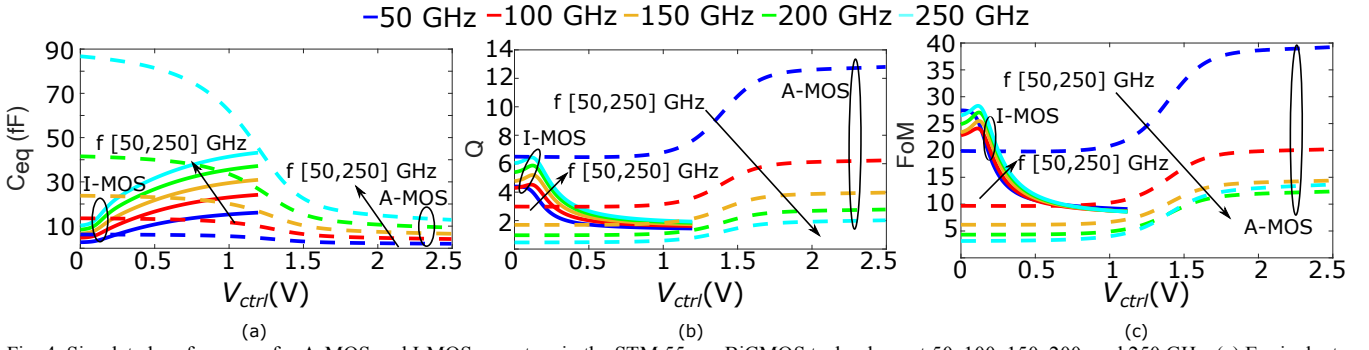
Fig. 4. Simulated performance for A-MOS and I-MOS varactors in the STM 55-nm BiCMOS technology at 50, 100, 150, 200, and 250 GHz. (a) Equivalent capacitance. (b) Q-factor. (c) Figure-of-Merit.
