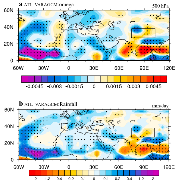
FIG. A7. Regressions of JJA-mean (a) vertical velocity (units: 10^{-2} \text{ Pa s}^{-1} ) and (b) rainfall (units: \text{mm day}^{-1} ) onto the normalized AMV index at decadal time scales in the ATL_VAR_AGCM simulations. Dotted shadings denote regressions significant at the 90% confidence level. The long-term linear trends for 1900–2013 in both variables were removed before the regression analyses.
