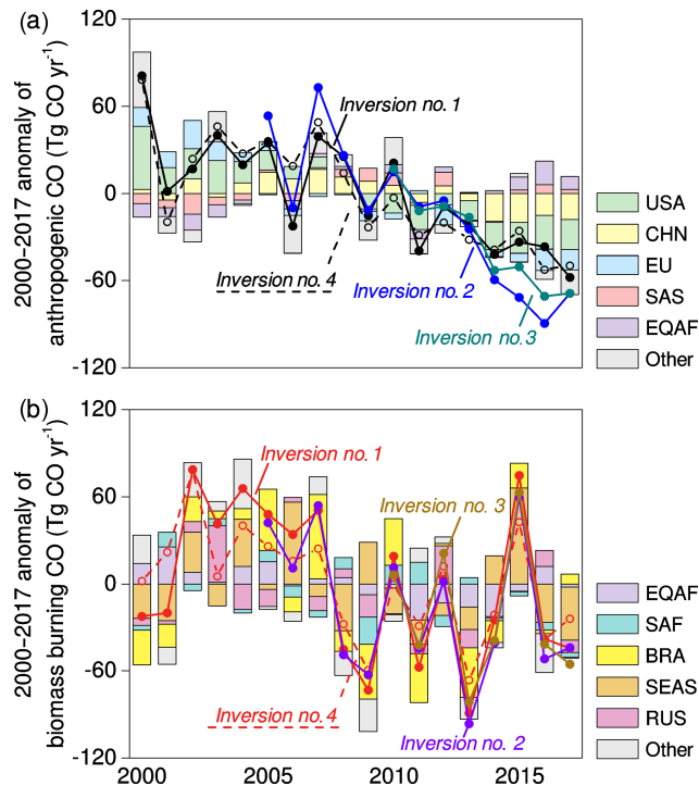
Figure 6. Global CO emission anomalies from 2000 to 2017. Anthropogenic (a) and biomass burning (b) emission anomalies are presented with global totals derived from Inversion nos. 1 to 4 (curves) as well as regional emission anomalies (stacked bar) derived from Inversion no. 1, including the top five emitters and the sum of all the other regions. For Inversion no. 1 and Inversion no. 4, the emission anomalies are calculated by removing the 2000–2017 average calculated from their own time series data. For Inversion no. 2 and Inversion no. 3, the emission anomalies are calculated by removing the 2000–2017 average calculated from Inversion no. 1.
