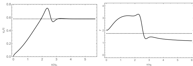
FIG. 1. Density dependence of the SV of stars v_s (left panel) and the polytropic index \gamma = d \ln P / d \ln \epsilon (right panel) in neutron matter.
